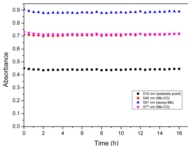
Figure 3. Change of absorption at selected wavelengths with increasing incubation time in the dark (0 to 16 h) for a solution of dendrimer 1 ( 4\ \mu\text{M} ) in 0.1 M PBS at pH 7.4 in the presence of myoglobin ( 60\ \mu\text{M} ) and sodium dithionite (10 mM) under a dinitrogen atmosphere as monitored by UV/vis spectroscopy.
