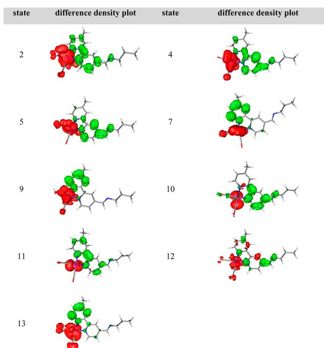
Figure 6. TDDFT difference densities for the most important singlet excitations for 3-A in the 300 to 600 nm range. Isosurface values are plotted at \pm 0.002 , with positive values shown in green and negative ones in red.
