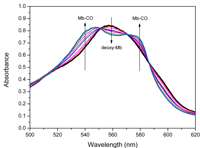
Figure 4. Change of absorption in the Q-band region of myoglobin with increasing irradiation time at 410 nm for a solution of dendrimer ( 4\ \mu\text{M} ) in 0.1 M PBS pH 7.4 in the presence of myoglobin ( 60\ \mu\text{M} ) and sodium dithionite (10 mM) under a dinitrogen atmosphere as monitored by UV/vis spectroscopy.
