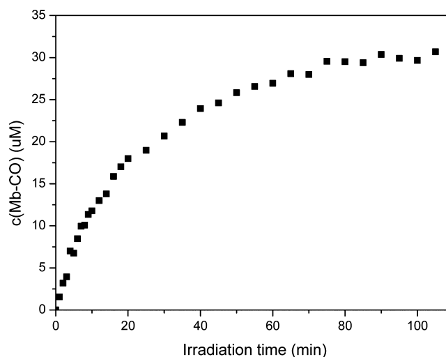
Figure 5. Amount of MbCO in \mu\text{M} formed with increasing irradiation time at 410 nm for a solution of compound 1 ( 4\ \mu\text{M} ) in 0.1 M PBS at pH 7.4 in the presence of myoglobin ( 60\ \mu\text{M} ) and sodium dithionite (10 mM) under a dinitrogen atmosphere as determined from UV/vis spectroscopy.
