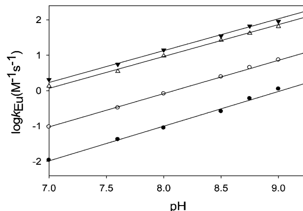
Figure 4. pH rate profile of second-order rate constants for cleavage of HpPNP by \text{Eu}(5) (●), \text{Eu}(3) (○), \text{Eu}_2(1) (▼), and \text{Eu}_2(2) (△). The solid lines through the values for second-order rate constants ( k_{\text{Eu}} ) show the theoretical fits of these data to the logarithmic form of eq 8.
