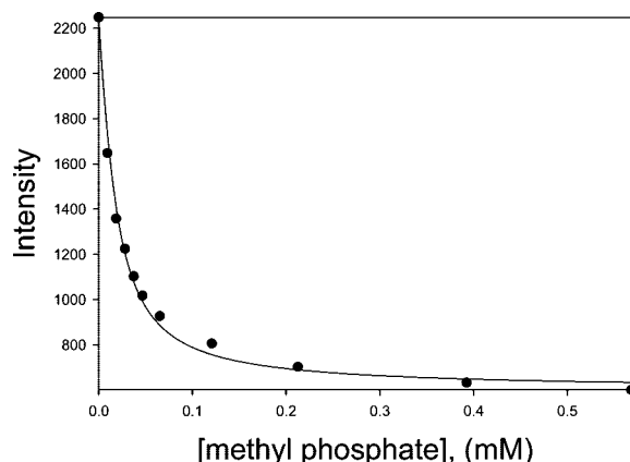
Figure 3. Plot of observed luminescent intensity (579.82 nm) of \text{Eu}_2(1) ( 3.30 \mu\text{M} ) as a function of total added MP concentration at 25^\circ\text{C} , I = 0.10 \text{ M NaNO}_3 , pH 7.6, 20 mM Hepes. The solid curve represents the best fit to eq 4 with K_d = 23 \mu\text{M} .
