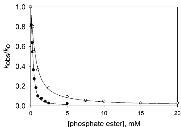
Figure 5. Diethyl phosphate ( DEP , \circ ) and monomethyl phosphate ( MP , \bullet ) inhibition of the \text{Eu}_2(\mathbf{1}) complex ( MP ( \bullet ), DEP ( \circ )) catalyzed cleavage of HpPNP at 25 °C, I = 0.10 M ( \text{NaNO}_3 ), pH 7.6, 20 mM Hepes buffer. Data is fit to eq 1 with K_i = 0.060 mM for MP and 0.43 mM for DEP .
