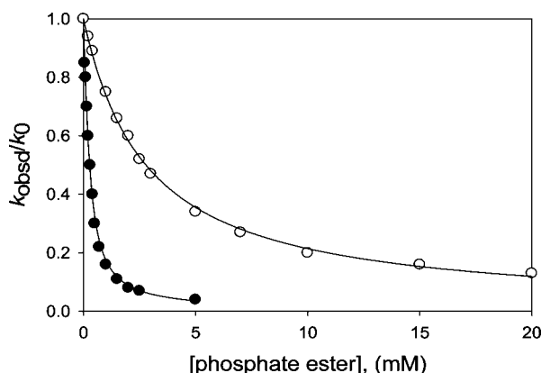
Figure 6. Diethyl phosphate ( DEP , \circ ) and monomethyl phosphate ( MP , \bullet ) inhibition of the \text{Eu}(\mathbf{3}) (0.2 mM) catalyzed cleavage of HpPNP at 25 °C, I = 0.10 M ( \text{NaNO}_3 ), pH 7.6, 20 mM Hepes. Data is fit to eq 1 with K_i = 2.7 mM for DEP and 0.18 mM for MP .
