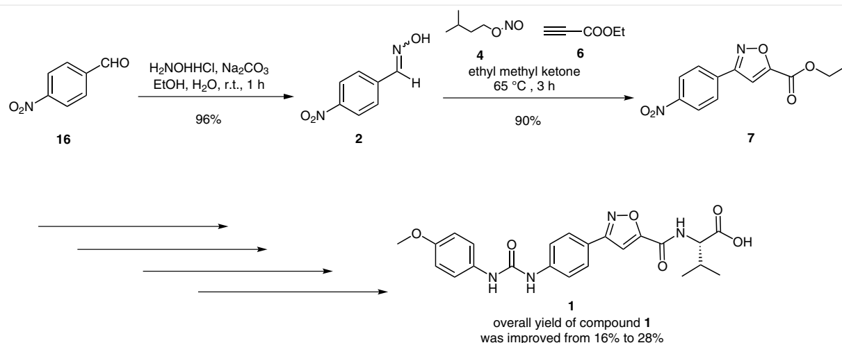
Scheme 5 Synthesis of 3-phenylisoxazole-5-carboxamide derivative 1 from isoxazole 7 with overall improved yield
