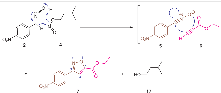
Scheme 6 Plausible reaction mechanism for the synthesis of isoxazole 7
