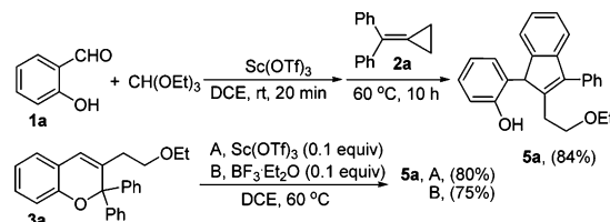
Scheme 1. Reactions at Higher Temperature
