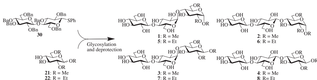
Figure 1. Syntheses of blockwise methylated or ethylated trisaccharide derivatives 1 – 8 .
