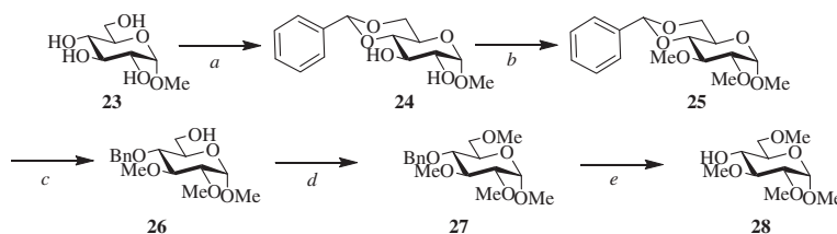
Figure 3. Synthetic route for methyl 2,3,6-tri-O-methyl- \alpha -D-glucopyranoside ( 28 ). (a) Benzaldehyde dimethylacetal/ p -TsOH/DMF/40 °C→80 °C/5 h/81.5%; (b) Mel/NaH/THF/rt/6 days/93.0%; (c) BH 3 -THF/TMSOTf/CH 2 Cl 2 /−40→0 °C/5 h/75.8%; (d) Mel/NaH/THF/40 °C/overnight/93.0%; (e) 10% Pd on C/THF/EtOH/under H 2 /rt/5 days/99.8%.
