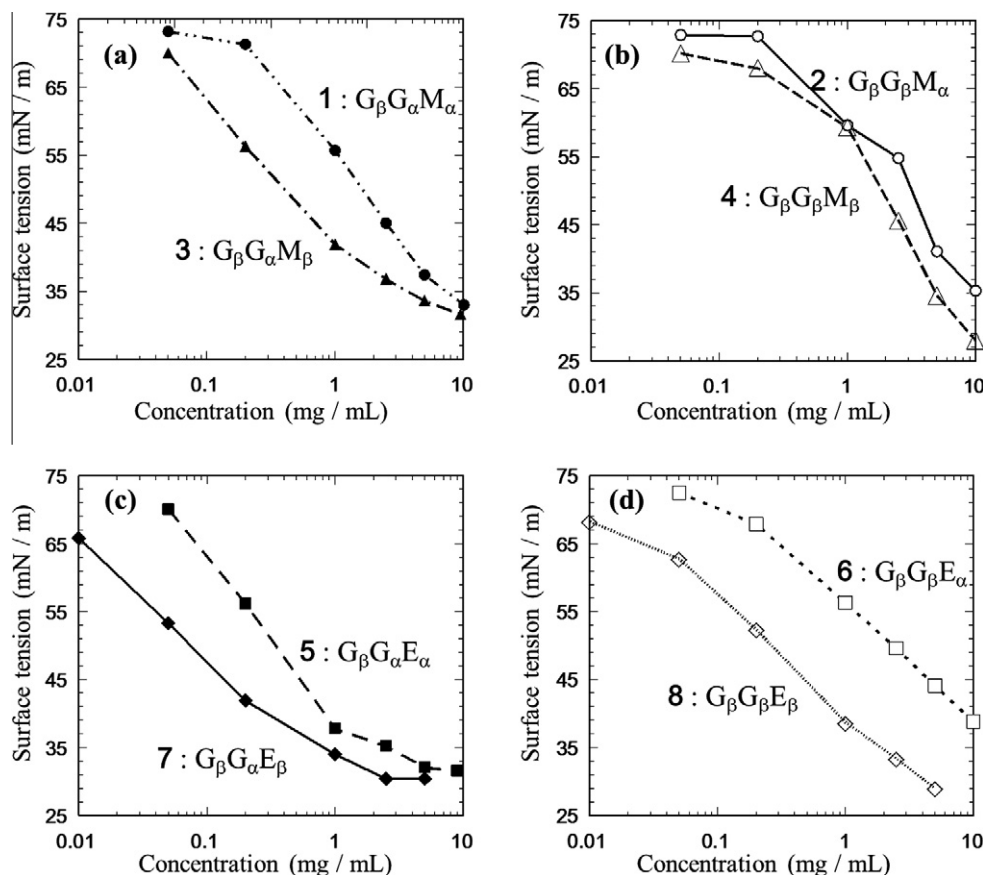
Figure 9. Surface tension–concentration curves of pure compounds 1–8 : the effect of \alpha - and \beta -linkages at C-1 on surface activity; \bullet : compound 1 ; \circ : compound 2 ; \blacktriangle : compound 3 ; \triangle : compound 4 ; \blacksquare : compound 5 ; \square : compound 6 ; \blacklozenge : compound 7 ; \diamond : compound 8 .
