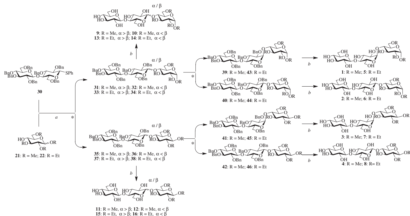
Figure 5. Synthetic routes for blockwise methylated or ethylated trisaccharide derivatives 1–16 . (a) NBS/AgOTf/MS 3 Å or MS 4 Å/EtCN or CH 2 Cl 2 /rt/under vacuum, (b) Pd(OH) 2 on C/THF/EtOH/under H 2 /rt. *Purification by a preparative thin layer chromatography (P-TLC).
