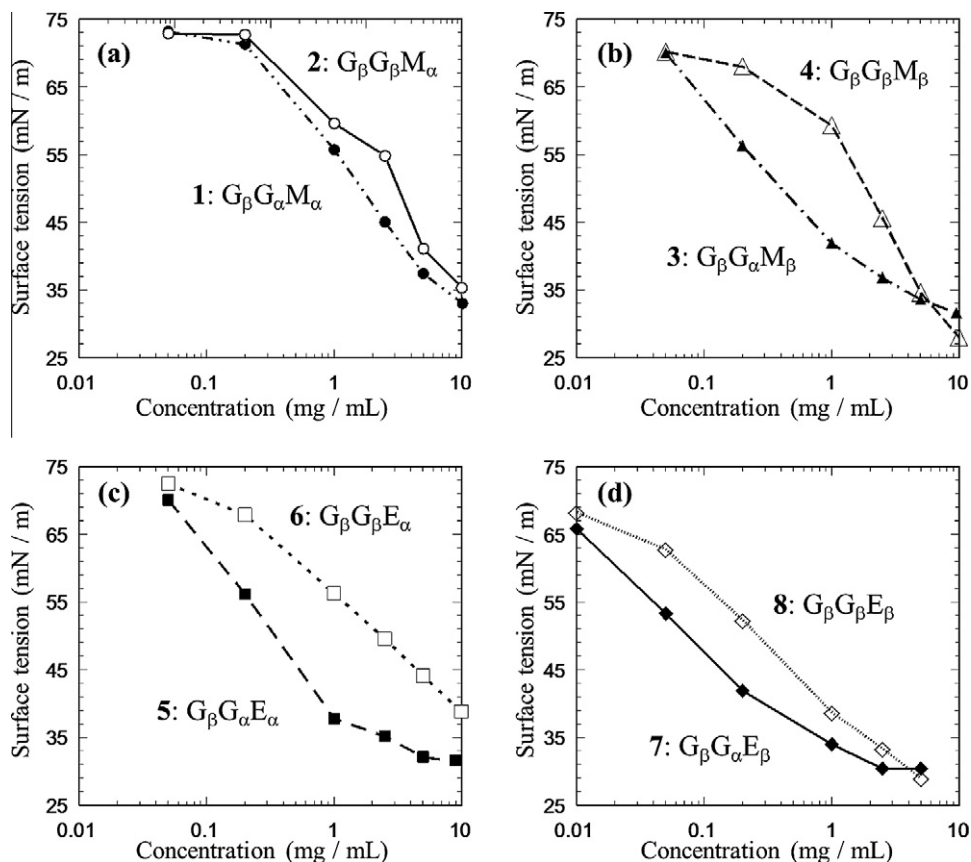
Figure 7. Surface tension–concentration curves of pure compounds 1–8 : the effect of \alpha - and \beta -(1 \rightarrow 4) linkages between hydrophobic and hydrophilic moieties on surface activity; \bullet : compound 1 ; \circ : compound 2 ; \blacktriangle : compound 3 ; \triangle : compound 4 ; \blacksquare : compound 5 ; \square : compound 6 ; \blacklozenge : compound 7 ; \diamond : compound 8 .
