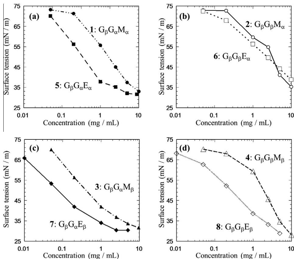
Figure 8. Surface tension–concentration curves of pure compounds 1–8 : the effect of methyl or ethyl group on surface activity; ●: compound 1 ; ○: compound 2 ; ▲: compound 3 ; △: compound 4 ; ■: compound 5 ; □: compound 6 ; ◆: compound 7 ; ◇: compound 8 .
