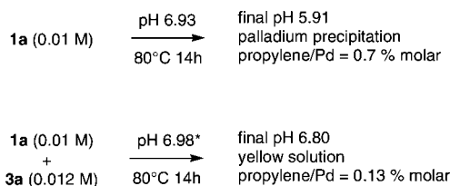
Figure 9. Beneficial effect of 3a on 1a stability. In the second reaction, 3a isomerization into 3b was observed ( 1.6\%/14 h: i.e., 0.11\% h -1 ). Without palladium, the 3a isomerization rate in a pH range 6.5–7.0 was estimated at 0.1\% and 0.38\% h -1 (see the Supporting Information).
