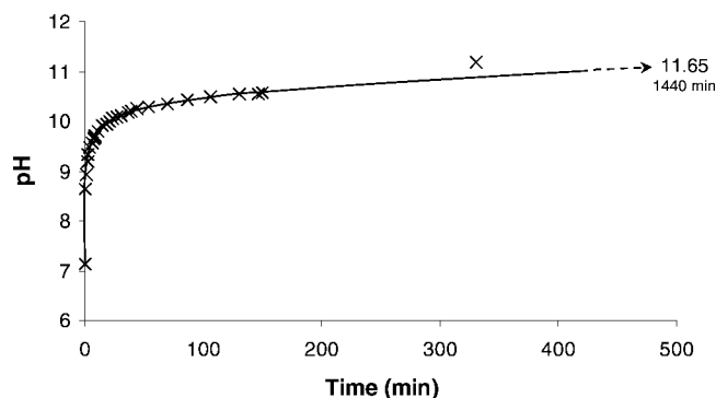
Figure 5. Allyl alcohol reaction without acid addition: pH versus time. Conditions: [Pd] = 0.0055 M in water at room temperature, allyl alcohol/Pd molar ratio 10, initial pH 7.14, final pH 11.65, close to the theoretical pH 11.74, after reaction [\text{OH}^-] = [\text{Pd}] = 0.0055 \text{ M} .
