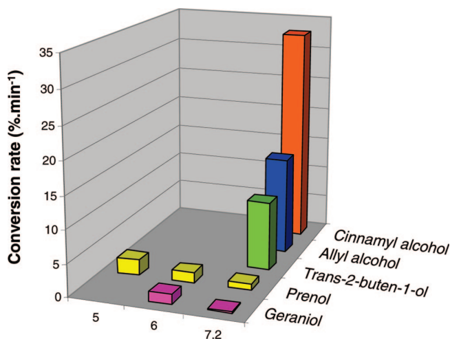
Figure 7. Comparative reactivity of allylic alcohols. Conditions: [\text{Pd}] = 0.0055 \text{ M} in water at 25^\circ\text{C} , initial pH 7, immediately after allylic alcohol addition, pH was maintained at 7 by 0.2 \text{ M HClO}_4 addition. Geraniol and cinnamyl alcohol were not totally soluble in water at the concentration 0.055 \text{ M} ; prenol and geraniol reactions, too slow at pH 7, were completed at a lower pH.
