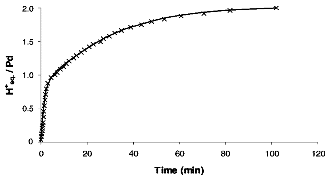
Figure 6. Rate of cinnamyl alcohol reaction with \text{Pd}(\text{TPPTS})_3 : \text{H}^+/\text{Pd} ratio versus time. Conditions: [\text{Pd}] = 0.0055 \text{ M} in water at 25^\circ\text{C} , cinnamyl alcohol/ \text{Pd} = 10 , initial pH 7, immediately after alcohol addition, pH was maintained at 7 by 0.2 \text{ M HClO}_4 addition.
