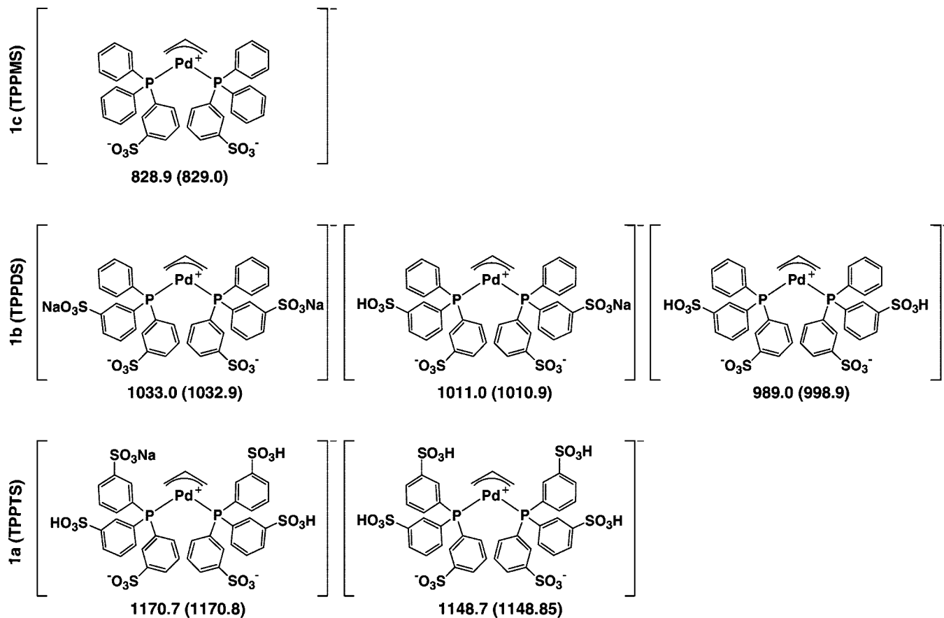
Figure 4. Selected negative-ion electrospray mass spectral data of ionic complexes 1c (TPPMS), 1b (TPPDS), and 1a (TPPTS).
