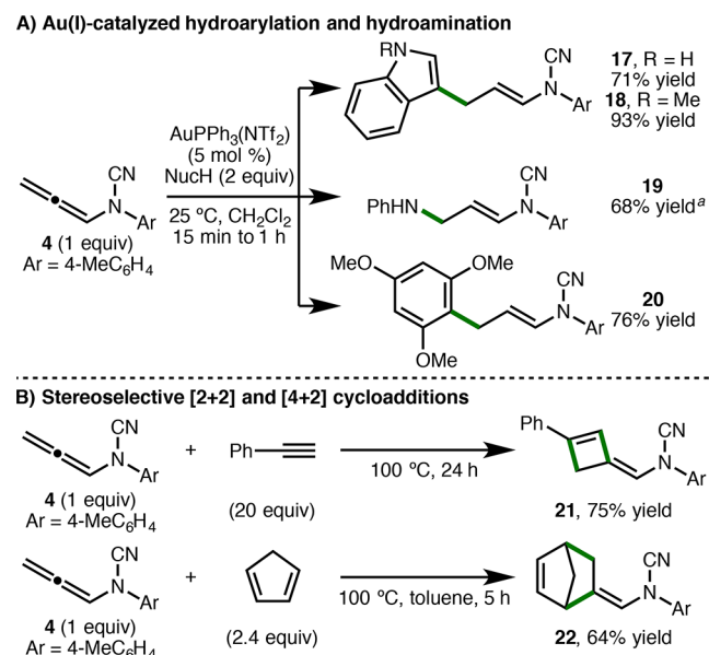
Scheme 5. Derivatization of N -Allenyl Cyanamides a
