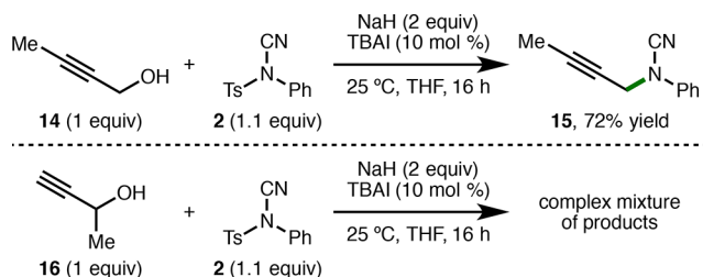
Scheme 4. Use of Substituted Propargyl Alcohols
