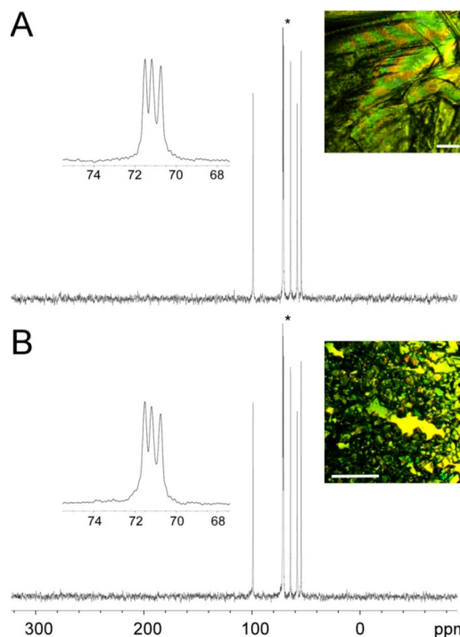
Figure 6. Representative CP-MAS 13 C NMR spectra of the MDM crystals in the absence and presence of AF(G)Ps. The CP-MAS 13 C NMR spectra of MDM crystals in the absence of AF(G)Ps (A) and in the presence of DAFP1 (B). The insets show the details of the peak with an asterisk and the habits of the MDM crystals are shown at the right upper corner of each panel (the length of the scale bars is 1 mm).
