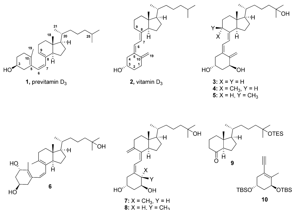
Figure 1. Structures of the 1,25-(OH) 2 D 3 , its metabolic precursors, the synthesized vitamin D 3 analogues, and their synthetic precursors.
