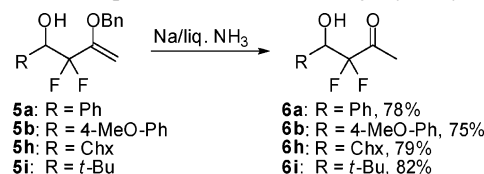
Scheme 3. Preparation of \alpha,\alpha -Difluoro- \beta -hydroxy Ketones
