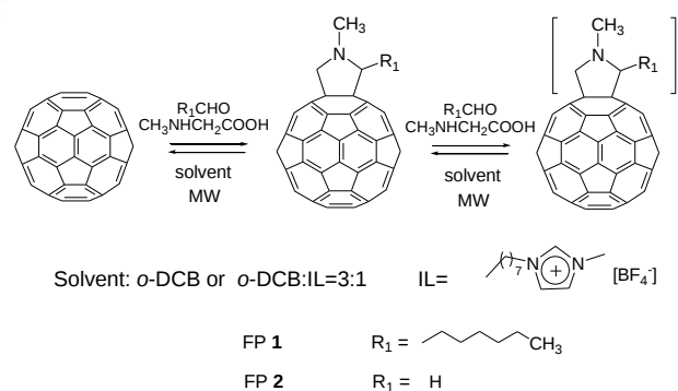
Scheme 1 Azomethine ylide cycloaddition to [60]fullerene yielding mono- and poly-adducts (FPs 1 and 2) by reacting heptaldehyde or formaldehyde respectively, under MW irradiation, in o-DCB/IL mixtures.
