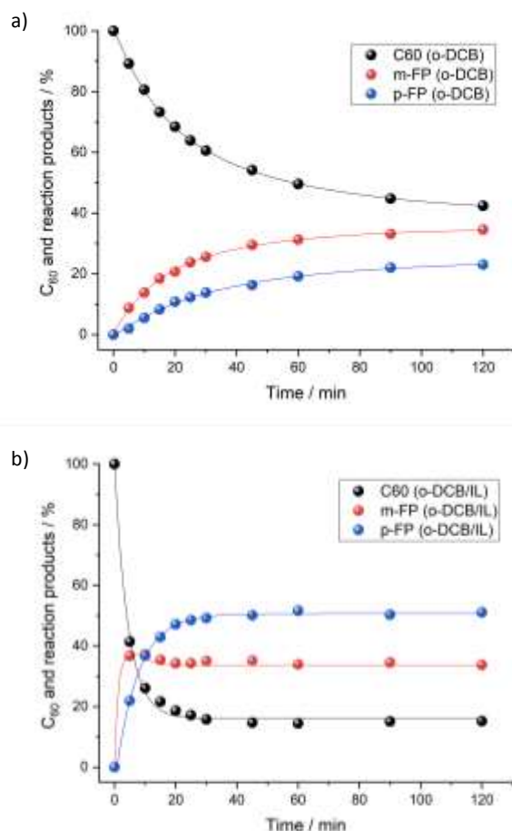
Figure 1. Kinetic traces of [60]fullerene conversion to m-FP 1 and p-FP 1 during 1,3-dipolar cycloaddition of sarcosine and heptaldehyde in 1 mL of o-DCB (a) or 0.8 mL of o-DCB/IL 3/1 v/v (b), at 423K. [60]fullerene 7 mM; sarcosine 14 mM, heptaldehyde 28 mM. Data are connected with continuous
