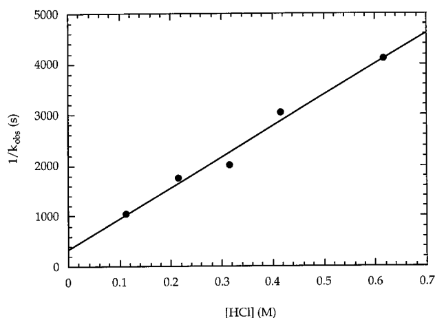
Figure 12. 1/ k obs vs [HCl] for reductive elimination of toluene from 6 in the presence of varying [HCl] and constant [HOTf]. For reaction conditions see Figure 5.
