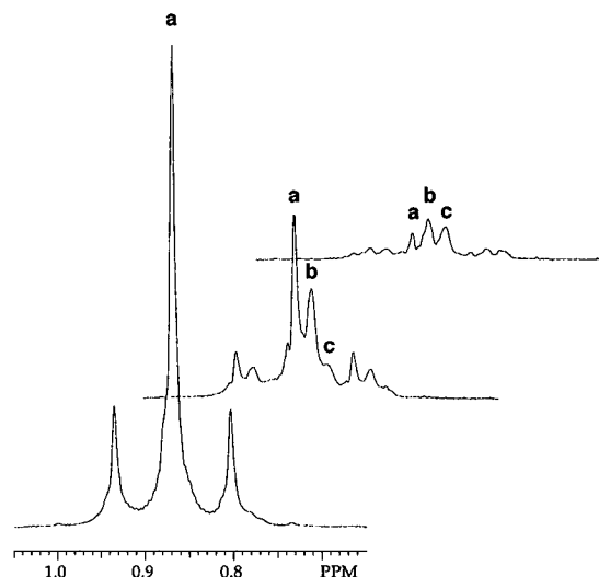
Figure 6. Sequence of ^1\text{H} NMR spectra demonstrating the appearance of shoulders upfield of the original \text{Pt(IV)}\text{--CH}_3 resonance from 12 in \text{CD}_3\text{OD} along with an overall decrease in the peak integration. The upfield shoulders are assigned as the sequentially deuterated methyl groups: a = \text{Pt--CH}_3 , b = \text{Pt--CH}_2\text{D} , and c = \text{Pt--CHD}_2 .
