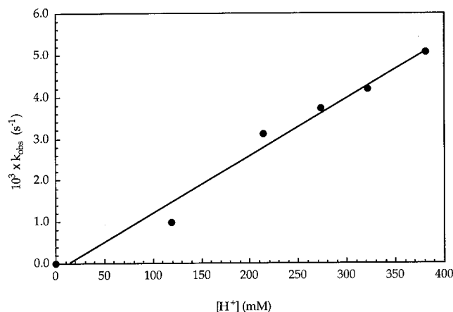
Figure 1. Plot of the [H^+] dependence of the rate of protonolysis of 2 in CD_3OD . [H^+] = 0 –32 equiv; [2] = 11.9 mM; [Cl^-] = 0 M; \mu = 1.0 M; temperature = -35 °C.
