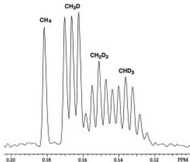
Figure 7. Full range of methane isotopomers that arise upon warming a reaction mixture containing 12 in \text{CD}_3\text{OD} prior to complete deuterium incorporation into the platinum–methyl groups.
