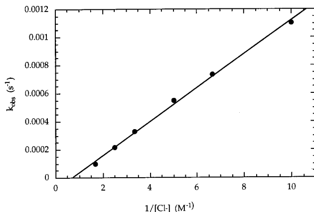
Figure 8. Plot of k_{\text{obs}} versus 1/[\text{Cl}^-] for deuterium incorporation into 12 in \text{CD}_3\text{OD}:\text{CD}_2\text{Cl}_2 (13:1). [\text{Cl}^-] = 0.10\text{--}0.60\text{ M} ; [\text{12}] = 21\text{ mM} ; [\text{H}^+] = 0.21\text{ M} ; \mu = 1.21\text{ M} ; temperature = -43\text{ }^\circ\text{C} .
