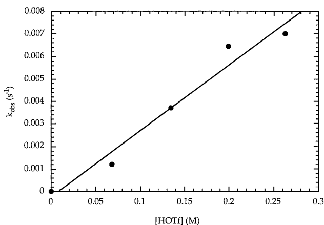
Figure 4. [HOTf] dependence of the rate of reductive elimination of toluene from 5 in \text{CD}_2\text{Cl}_2 . [HOTf] = 0–20 equiv (relative to [ 6 ]); [ 6 ] = 13 mM; [HCl] = 65 mM; temperature = -61 °C.
