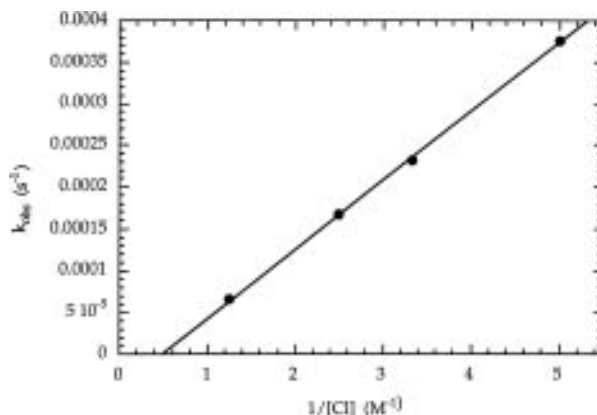
Figure 9. Plot of k_{\text{obs}} versus 1/[\text{Cl}^-] for methane elimination from 12 in \text{CD}_3\text{OH}:\text{CD}_2\text{Cl}_2 (13:1). [\text{Cl}^-] = 0\text{--}0.80\text{ M} ; [\text{12}] = 21\text{ mM} ; [\text{H}^+] = 0.21\text{ M} ; \mu = 1.21\text{ M} ; temperature = -28\text{ }^\circ\text{C} .
