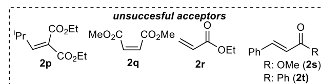
Scheme 2 Scope of electron-deficient alkenes. a Isolated pure product. b 1.7:1 MeOH/EtOAc (0.185 M) was used as solvent mixture to improve the solubility of substrates. c 3 equiv of volatile MVK were used.
