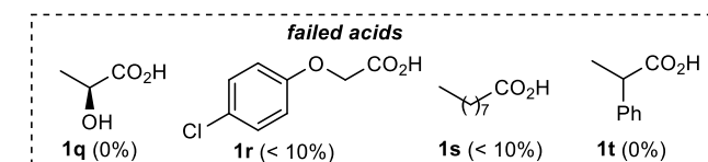
Scheme 3. Scope of acids. a Isolated pure product. b 2 equivalents of acid 1 were used. c Another portion of photocatalyst (2.5 mol %) was added after 48 h. d Another portion of acid 1 (1.5 equiv.) was added after 48 h. e See SI for details.
