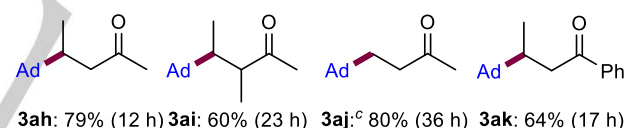
Scheme 1. (a) Plausible mechanism for a photoredox neutral decarboxylative Giese-type reaction catalyzed by [\text{Acr}^+-\text{Mes}] and base. (b) Previous work.
