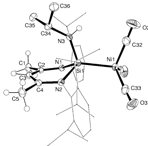
Figure 7. Molecular structure of 23b with thermal ellipsoids drawn at the 50% probability level. Hydrogen atoms are omitted for clarity, except those of C1, C3, C5, and N3. Selected bond distances (pm) and angles (deg) of 23b : Si1–Ni1, 225.52(6); Si1–N1, 186.2(1); Si1–N2, 183.8(1); Si1–N3, 173.0(2); N1–C2, 133.7(2); C1–C2, 150.0(2); C2–C3, 139.4(2); C3–C4, 138.6(2); C4–C5, 150.6(3); N2–C4, 134.3(2); Ni1–C(average), 178.3; C–O(average), 113.7; N1–Si1–N2, 94.11(6); N1–Si1–Ni1, 117.76(5); N3–Si1–Ni1, 114.83(6); N1–Si1–N3, 104.11(7).
