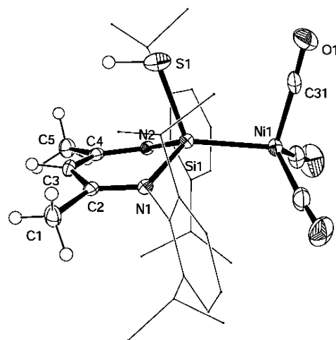
Figure 5. Molecular structure of 17 with thermal ellipsoids drawn at the 50% probability level. Hydrogen atoms are omitted for clarity, except those of C1, C3, and S1. Selected bond distances (pm) and angles (deg) of 17 : Si1–Ni1, 224.66(6); Si1–S1, 219.01(9); Si1–N1, 184.0(2); Si1–N2, 184.4(2); N1–C2, 134.6(3); C1–C2, 150.2(4); C2–C3, 138.6(3); C3–C4, 138.9(3); C4–C5, 150.2(4); C4–N2, 134.7(3); Ni1–C(average), 178.5; C–O(average), 114.1; N1–Si1–N2, 95.67(9); N1–Si1–Ni1, 120.88(7); Ni1–Si1–S1, 113.50(3); N1–Si1–S1, 100.35(7).
