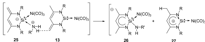
Scheme 8. Proposed Intermediates during the Formation of 23a–c with Simultaneous Activation of Amines R'NH_2^a
