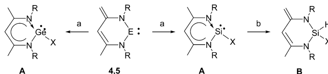
Scheme 1. Reaction Pathways of Germylene 4 and Silylene 5 with HX a
