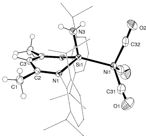
Figure 6. Molecular structure of 23a with thermal ellipsoids drawn at the 50% probability level. Hydrogen atoms are omitted for clarity, except those of C1, C3, and N3. Selected bond distances (pm) and angles (deg) of 23a : Si1–Ni1, 225.5(1); Si1–N1, 185.2(2); Si1–N2, 171.1(4); N1–C2, 134.0(4); C1–C2, 150.8(4); C2–C3, 138.8(3); Ni1–C(average), 178.6; C–O(average), 114.0; N1–Si1–N1, 94.06(9); N1–Si1–Ni1, 120.98(8); N3–Si1–Ni1, 100.5(2); N1–Si1–N3, 100.5(2).
