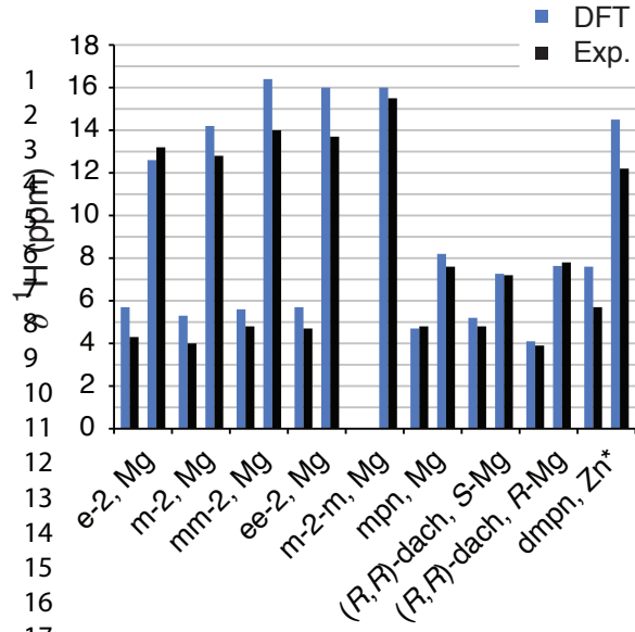
(a) ^1\text{H} : RMSD = 1.3 ppm
