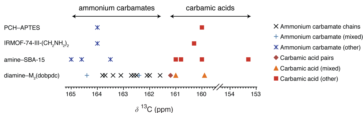
Figure 6. Summary of reported ^{13}\text{C} chemical shifts for chemisorbed \text{CO}_2 species in amine-functionalized adsorbents. Data for diamine- \text{M}_2(\text{dobpdc}) samples are from this work and Refs 15 and 19; data for amine-functionalized SBA-15 materials are from Refs 35, 41, and 45; data for IRMOF-74-III- (\text{CH}_2\text{NH}_2)_2 are from Ref 40 ; and data for PCH-APTES (porous clay heterostructure functionalized with 3-aminopropyltriethoxysilane) are from Ref 44 . For discussion of mixed chemisorption structures, see below.
