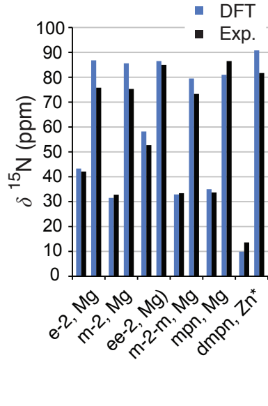
(c) ^{15}\text{N} : RMSD = 6.3 ppm
