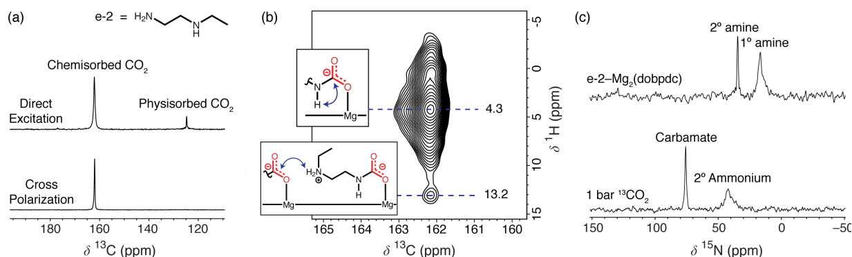
Figure 3. Solid-state MAS NMR (16.4 T) spectra of e-2-Mg 2 (dobpdc)-CO 2 . (a) 13 C NMR spectra by direct excitation (no 1 H decoupling) and cross-polarization (with continuous wave decoupling of 1 H). A 1:1 CO 2 :diamine reaction affords a capacity of 4.0 mmol/g CO 2 , which is reached above the adsorption step of the material (see Figure S1). Cross-polarization experiments allow the much faster observation of chemisorbed CO 2 compared to direct excitation experiments (partly because of the long longitudinal relaxation time, T 1 = 60 s, for chemisorbed CO 2 ). Cross-polarization is used for the majority of 13 C experiments that follow in this work. Note that framework and amine carbons are only weakly observed in these experiments, as they have the natural abundance of 13 C (~1%). (b) 1 H → 13 C HETCOR (contact time 100 μs) spectrum and correlation assignments. (c) Nitrogen-15 NMR spectra (natural isotopic abundance) of e-2-Mg 2 (dobpdc) before and after reaction with 13 CO 2 (1 bar). Recent X-ray crystallography of toluene-solvated e-2-Zn 2 (dobpdc) showed that this diamine binds to zinc(II) from the 1° amine, 14 with dynamics in the anticipated 1° amine-Mg interaction a likely cause of 15 N line broadening for the 1° amine 15 N resonance here. The magic angle spinning (MAS) rate was 15 kHz in all cases. 13 CO 2 gas dosing pressures were approximately 1 bar, and gas dosing and NMR experiments were performed at room temperature.
