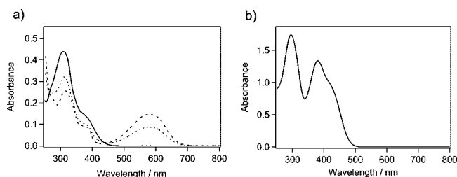
Figure 2. (a) Photochromic spectral change of 1 in \text{CH}_2\text{Cl}_2 . Solid line: open-ring isomer 1a ; dashed line: closed ring isomer 1b ; dotted line: in the photostationary state under irradiation with 313 nm light. (b) Absorption spectrum of 2a in \text{CH}_3\text{CN} . 2a is photoinactive.
