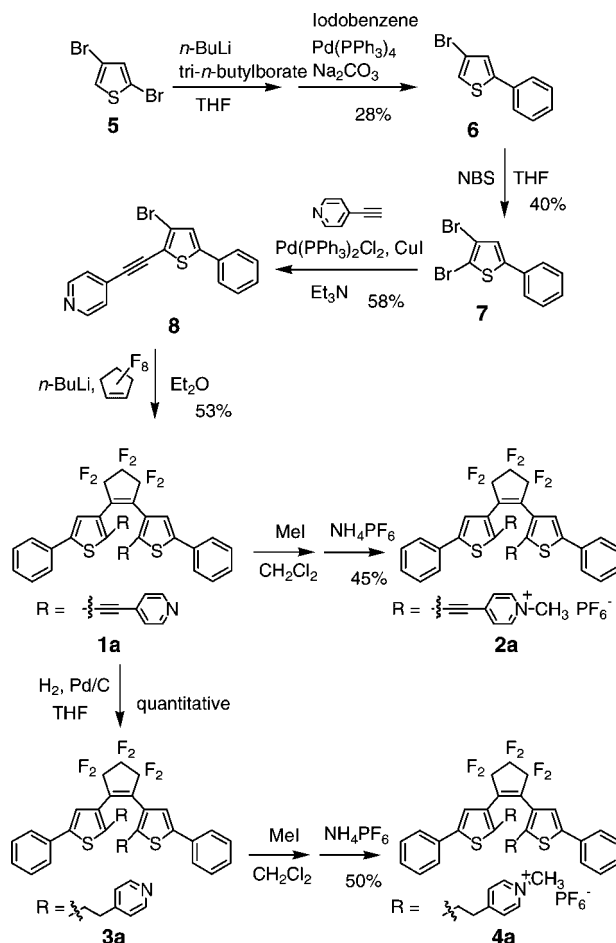
Scheme 1. Synthesis of Diarylethenes 1a–4a
