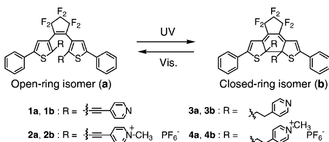
Figure 1. Diarylethenes with (4-pyridyl)ethynyl and (4-pyridyl)ethyl groups.
