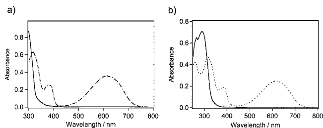
Figure 3. Photochromic spectral change of (a) 3a in \text{CH}_2\text{Cl}_2 and (b) 4a in \text{CH}_3\text{CN} . Solid line: open-ring isomers 3a and 4a ; dashed line: closed ring isomer 3b ; dotted line: in the photostationary state under irradiation with 313 nm light. 4b could not be isolated.
