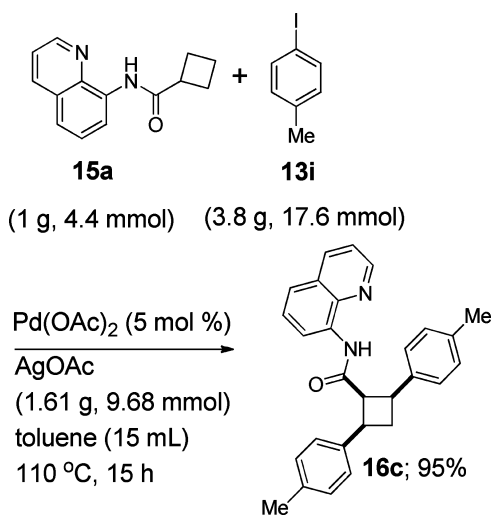
Scheme 10. Gram Scale Double C–H Arylation of 15a
