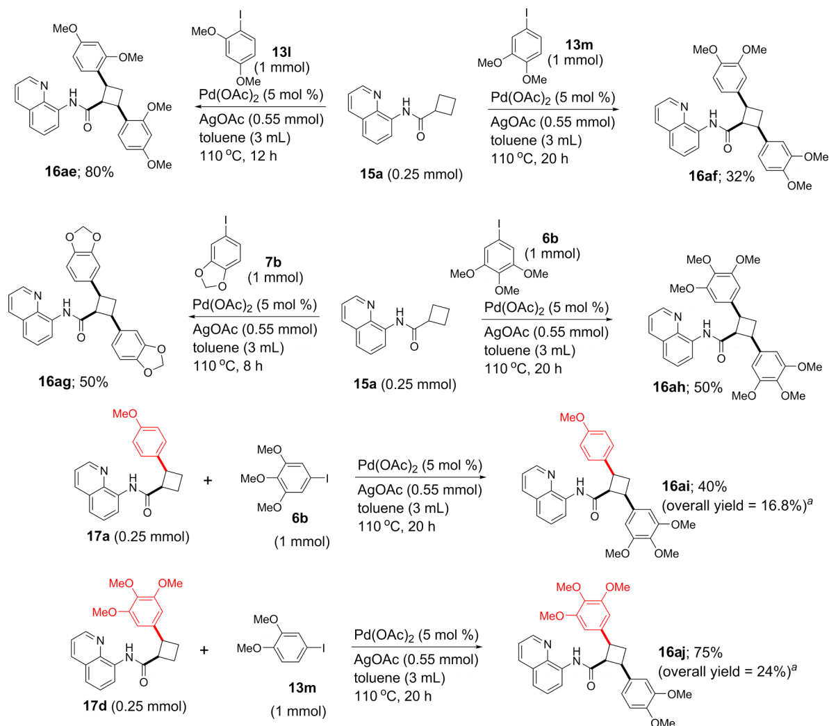
Scheme 9. Scope and Synthesis of Cyclobutane Derivatives Analogous to Cyclobutane Natural Products. a
