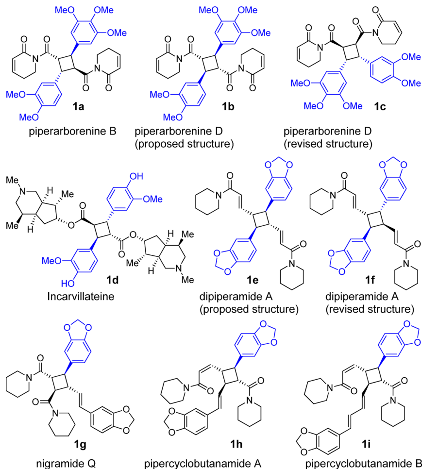
Figure 1. Representative cyclobutane natural products.
