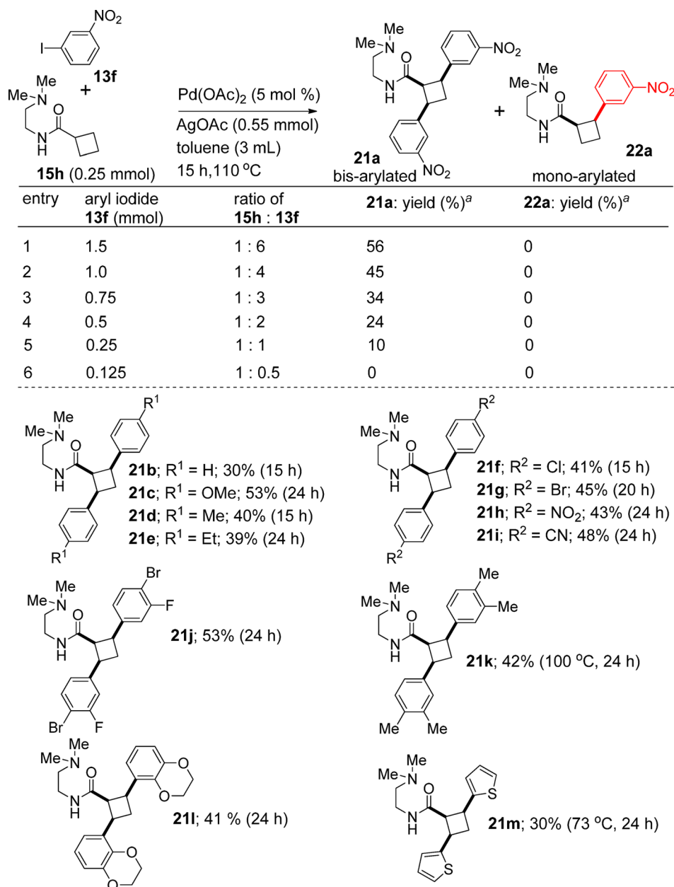
Scheme 7. Investigation of the Pd-Catalyzed C–H Arylation of N -(2-(Dimethylamino)ethyl)-cyclobutanecarboxamide. a,b
