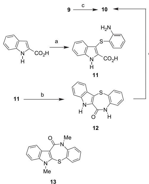
Scheme 4. Confirmation of structures of 9 and 10 . Reagents and conditions: (a) 2,2'-diaminodiphenyldisulfide, NaH, DMF (93%); (b) SiO 2 , toluene, reflux (63%); (c) n -Bu 4 NHSO 4 , 50% NaOH, CH 3 I, toluene, reflux [from 9 (76%), from 12 (89%)].
