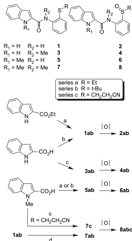
Scheme 2. Synthesis of 2-indoleanilides. Reagents and conditions (compound number, % yield): (a) 2-ethylthioaniline, AlMe 3 , toluene, reflux ( 1a 92%, 5a 84%); (b) SOCl 2 , Et 2 O, 2-(alkylthio)aniline, rt ( 1a , 32%, 1b 71%, 5b 59%); (c) SOCl 2 , Et 2 O, N -methyl-2-(alkylthio)aniline, rt ( 3a 38%, 3b 79%, 7c 27%); (d) 50% NaOH, CH 3 I, n -Bu 4 NHSO 4 , toluene ( 7a 82%, 7b 79%).
