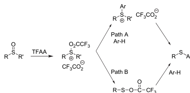
Scheme 1. Sulfenylation pathway depends upon the timing of events.
