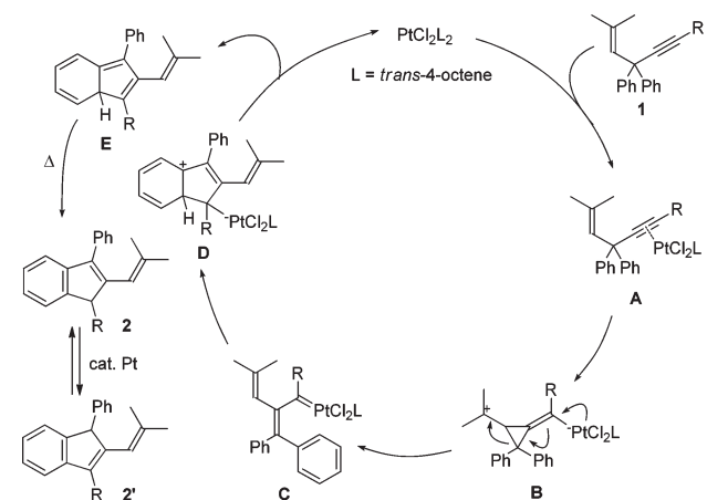
Scheme 3. Proposed Mechanism
