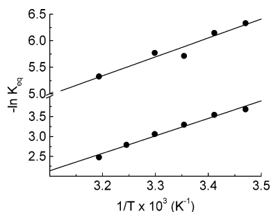
Figure 3. Plots of -\ln K vs 1/T for the reactions of cis - \text{PtCl}_2(\text{CO})_2 with cyclohexene (eq 3, upper plot) and with 1-octene (eq 4) in 1,2-dichloroethane.
