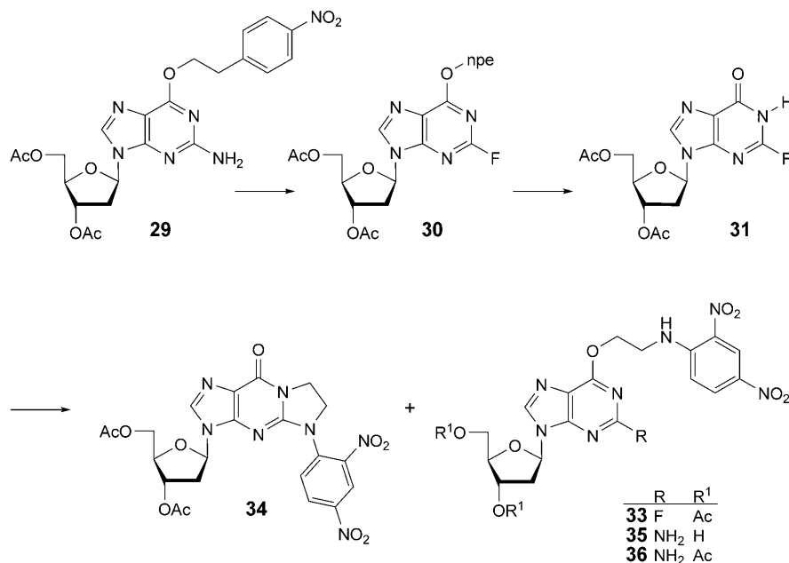
Scheme 4
