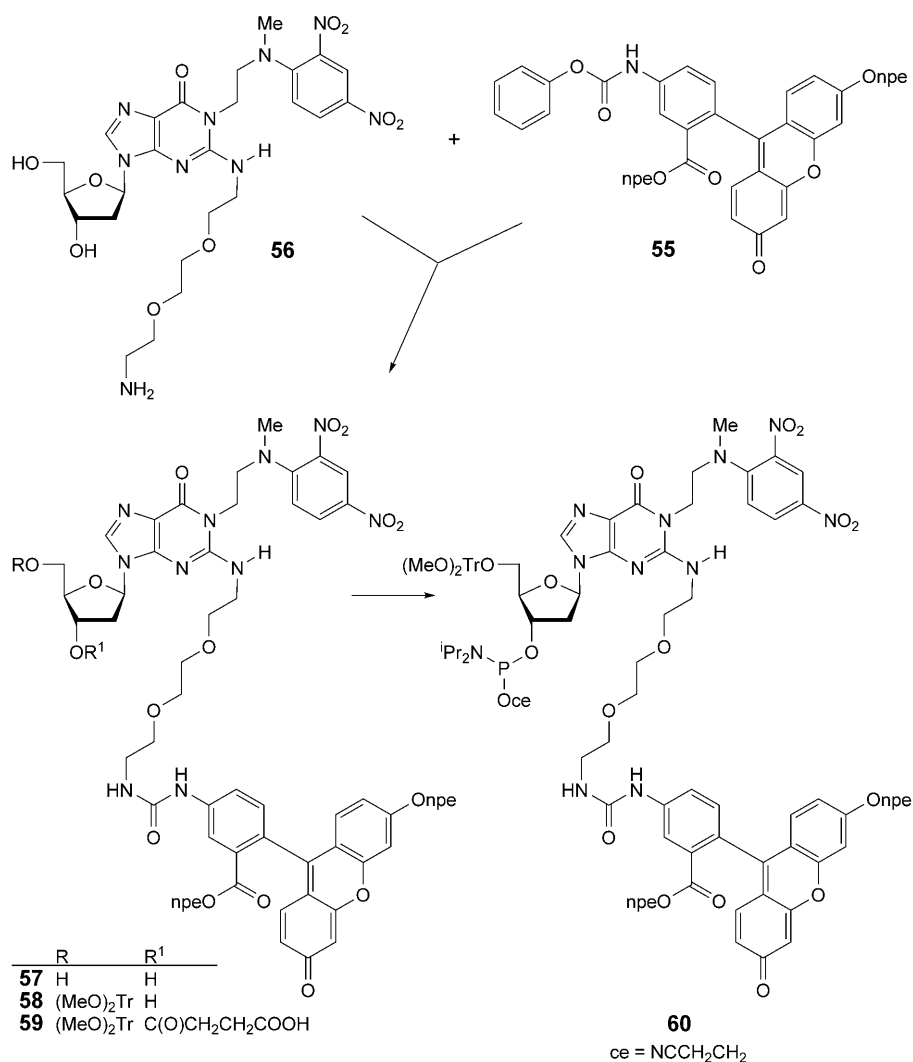
Scheme 6
