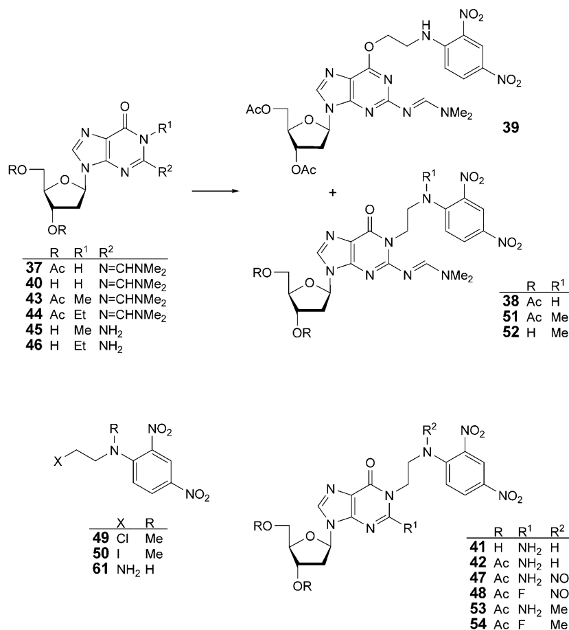
Scheme 5
