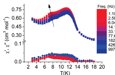
Figure 4. Plot of \chi' (upper) and \chi'' (lower) vs T for 2 at variable frequencies. The dotted arrow highlights the occurrence of a second, frequency-dependent feature around 8 K.
