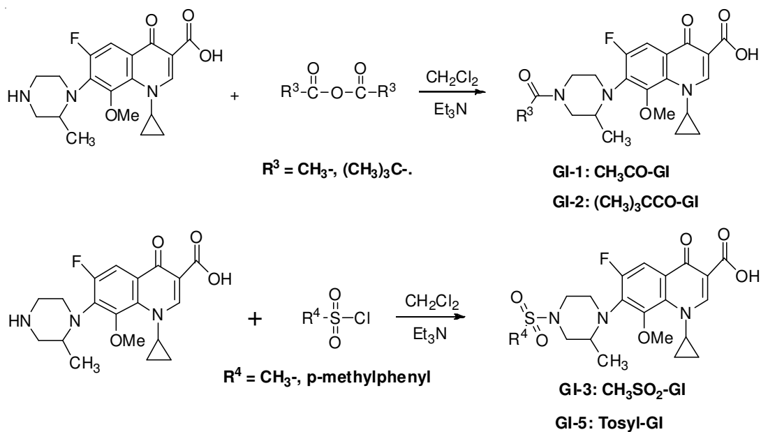
Scheme-IV: Synthetic route of compound GI-1, GI-2, GI-3 and GI-5
