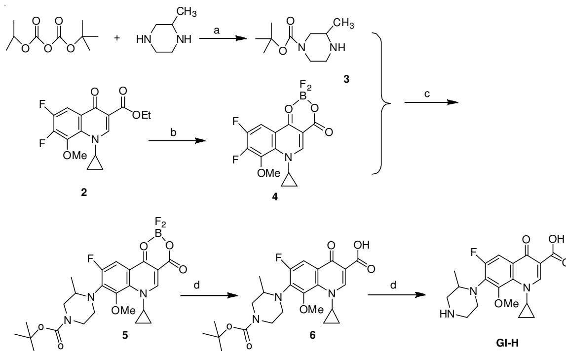
Scheme-I: Reactions and conditions: (a) di- tert -butyl dicarbonate (1 equiv), 2-methylpiperazine (1 equiv), CH 2 Cl 2 , 0 °C, 1h, 93 % for 3 ; (b) BF 3 ·Et 2 O (13 equiv), ethyl ester derivative (1 equiv), THF, reflux, 2d, 56 % for 4 ; (c) boron chelate-type intermediate (1 equiv), Boc-protected 2-methylpiperazine (2.1 equiv), DMSO, 0 °C, 0.5 h, then 40 °C, 3d, 23 % for 5 ; (d) CH 3 OH, reflux, 12 h, then 0 °C, HCl(aq), 0.5 h, 40 % for GI-H
