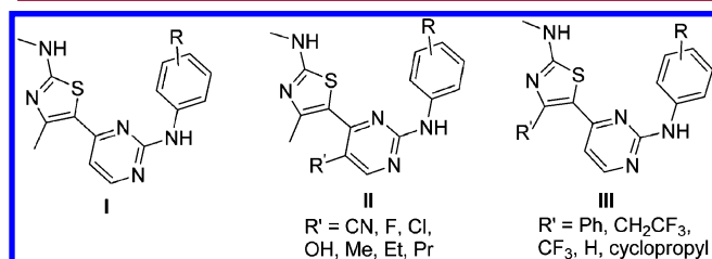
Figure 1. 4-(Thiazol-5-yl)-2-(phenylamino)pyrimidine derivatives.
