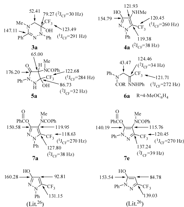
Chart 5. 13 C-NMR Chemical Shifts of Representative Heterocycles Prepared in This Work and Two Related Pyrazoles
