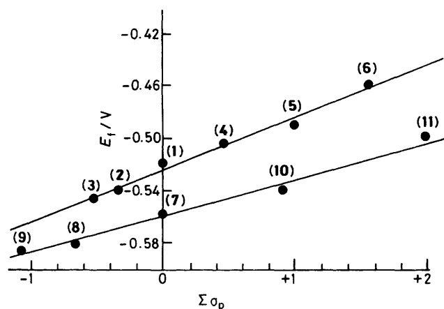
Figure 4. Plot of E_f^1 vs. \Sigma\sigma_p for the mononuclear complexes (1)–(11)
