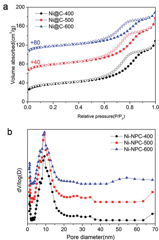
Fig. 6 (a) N_2 absorption-desorption isotherms and (b) their corresponding pore size distributions ( N_2 absorption-desorption isotherms for Ni@C-500 and Ni@C-600 are vertically offset by 40 and 80 cm^3 g^{-1} ).
