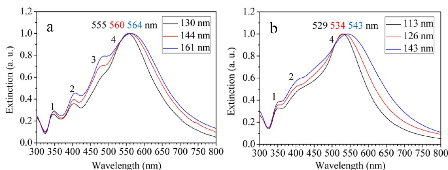
Figure 7. UV–vis absorption spectra of Au–Ag core–shell (a) nanocubes and (b) octahedra with different sizes. Body diagonals are used for particle size.
