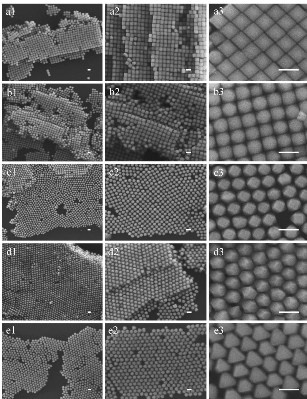
Figure 2. SEM images of Au–Ag core–shell (a1–a3) nanocubes, (b1–b3) truncated cubes, (c1–c3) cuboctahedra, (d1–d3) truncated octahedra, and (e1–3) octahedra viewed at different magnifications. All scale bars are equal to 100 nm.
