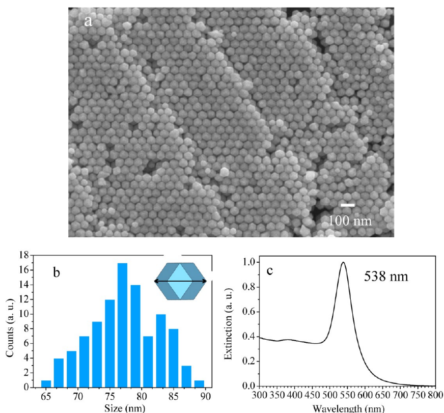
Figure 1. (a) SEM image of the synthesized rhombic dodecahedral gold nanocrystals. (b) Size distribution histogram and a drawing of the particle. The arrow indicates the particle size. (c) UV-vis absorption spectrum of the rhombic dodecahedral gold nanocrystals.
