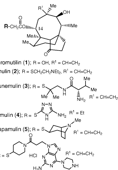
Figure 1. Pleuromutilin derivatives.
