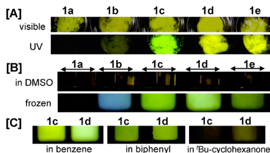
Figure 4. Photographs of fluorescence for 1a–e . [A] Pictures of solid 1a–e under visible light (top panel) and 365 nm UV light (bottom panel). [B] Pictures of 1.0 \times 10^{-3} M DMSO solutions of 1a–e under 365 nm UV light (top) and those of the frozen state (bottom). [C] Pictures of frozen solutions of 1c and d in benzene ( 1.0 \times 10^{-3} M), biphenyl ( 1.0 \times 10^{-3} mol/kg), and 4- t -butylcyclohexanone ( 1.0 \times 10^{-3} mol/kg) under 365 nm UV light. The DMSO and benzene solutions were prepared at rt and then frozen at -20 °C. The biphenyl and 4- t -butylcyclohexanone solutions were prepared at 90 °C and then solidified at rt.
