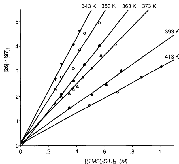
Figure 1. Plots of [\text{26}]_f/[\text{27}]_f vs. [(\text{TMS})_3\text{SiH}]_0 for the reaction of 23 with \approx 20 molequiv of (\text{TMS})_3\text{SiH} . The slopes ( k_{\text{H}}/k_{\text{re}} ) and intercepts ( k_{\text{rc}}/k_{\text{re}} ) are reported in Table 1.
