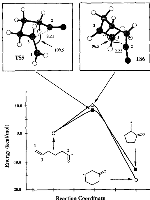
Figure 3. Schematic diagram showing the energy barriers for the 5- exo and 6- endo -cyclizations obtained by CASPT 2N. The energies of the reactant and products refer to the linear and chair arrangements, respectively. The inserts show some important features of the optimized transition structures.
