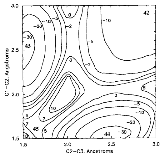
Figure 4. Potential energy surface linking structures 42 , 43 , 44 , and 45 of Scheme 7, as obtained by AM1 with the C. I. = 2 option. The lines of equal energy are calculated \Delta H_f^\circ in kcal mol −1 for the specified C1–C2 and C2–C3 distances with full optimization of all other geometric parameters. Scheme 7 gives the numbering designations for C1, C2, and C3.
