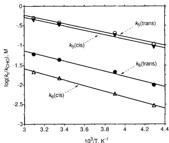
Figure 2. Arrhenius plots for the k_5/k_{\text{CHO}} ratios obtained at various temperatures for the cyclization of acyl radical 30 .
