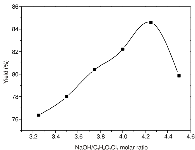
Fig. 3. Effect of NaOH/C 3 H 4 Cl 2 O 2 molar ratio on the yield of glyoxalic acid
