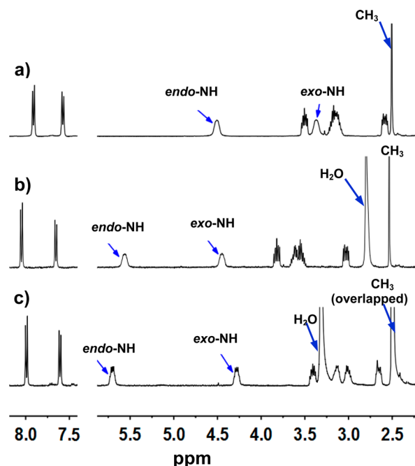
Figure 5. ^1\text{H} NMR spectra of [\text{Re}(\text{CO})_3(\text{N}(\text{SO}_2\text{tol})\text{dien})]\text{PF}_6 ( 6 ), illustrating the relative position of NH signals observed at 25 °C in (a) acetonitrile- d_3 , (b) acetone- d_6 , and (c) \text{DMSO-}d_6 .
