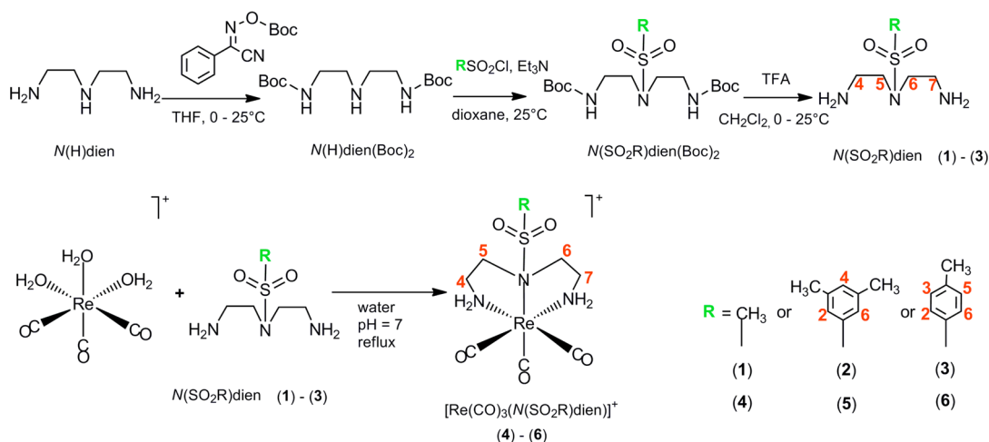
Figure 1. General reaction scheme for the synthesis of N(\text{SO}_2\text{R})\text{dien} ligands (top) and [\text{Re}(\text{CO})_3(N(\text{SO}_2\text{R})\text{dien})]^+ complexes (bottom).
