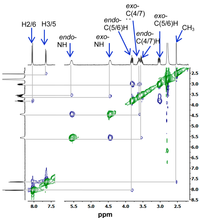
Figure 6. ^1\text{H} - ^1\text{H} ROESY spectrum of [\text{Re}(\text{CO})_3(\text{N}(\text{SO}_2\text{tol})\text{dien})]\text{PF}_6 ( 6 ) in acetone- d_6 at 25 °C. An expanded version of this figure is in Supporting Information (Figure S6).
