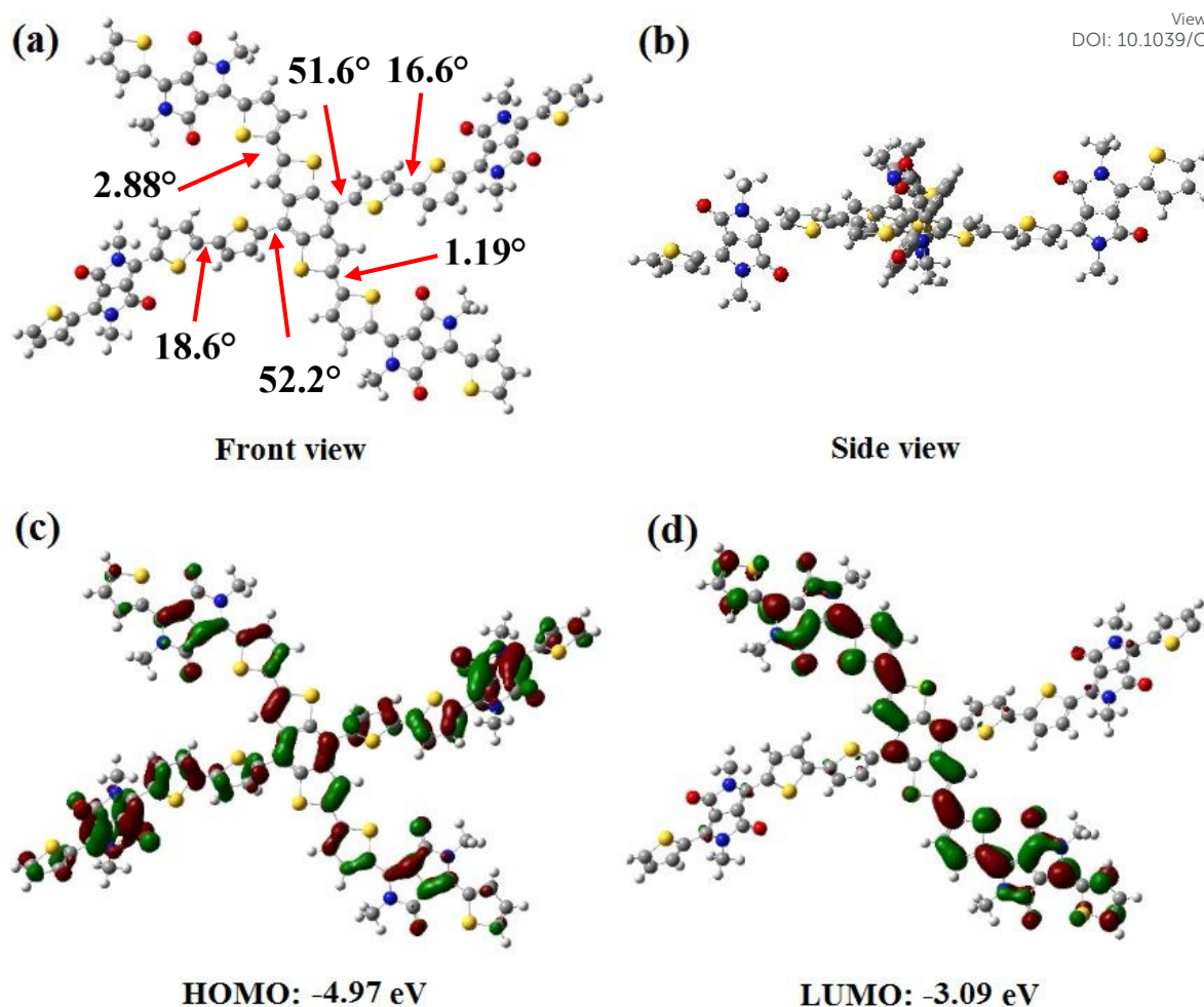
Fig. 2 (a, b) Optimized geometry and (c, d) frontier molecular orbitals of BDT(DPP) 4 .
