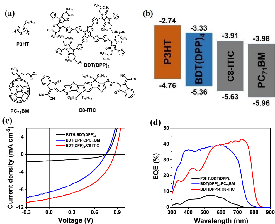
Fig. 4 (a) chemical structures and (b) Energy levels of P3HT, BDT(DPP) 4 , C8-ITIC and PC 71 BM, (c) J - V curves and (d) EQE spectra of OSC devices based on P3HT:BDT(DPP) 4 , BDT(DPP) 4 :PC 71 BM and BDT(DPP) 4 :C8-ITIC.
