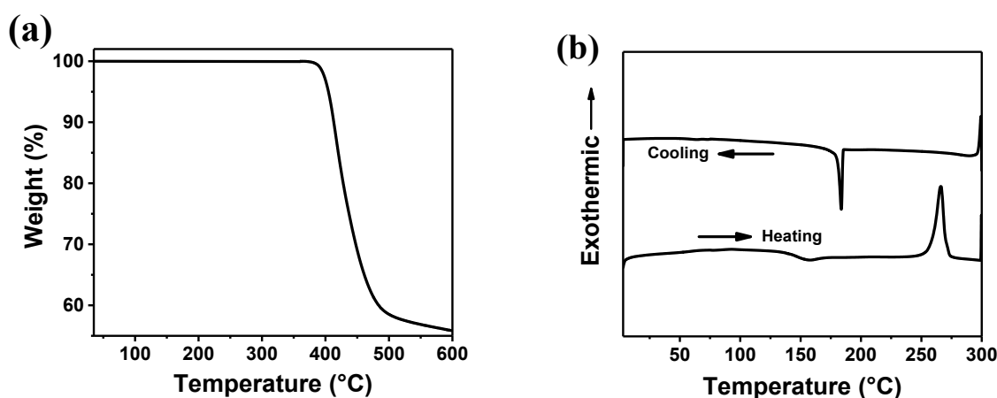
Fig. 1 (a) TGA and (b) DSC curves of \text{BDT}(\text{DPP})_4 at a heating/cooling speed of 10\text{ °C min}^{-1} under \text{N}_2 .
