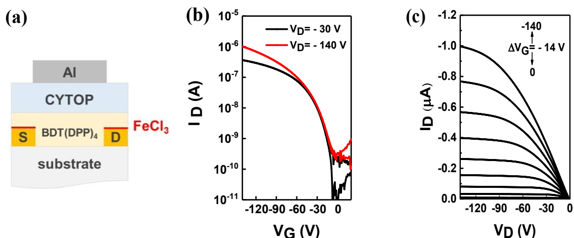
Fig. 5 (a) The top-gate, bottom-contact (TG-BC) transistor architecture employed in this work. (b) Typical transfer characteristics at V_D = -30 V and V_D = -140 V. (c) Output characteristics measured for the same transistor. Transistor channel length ( L ) and width ( W ) were 30\ \mu\text{m} and 1\ \text{mm} , respectively.
