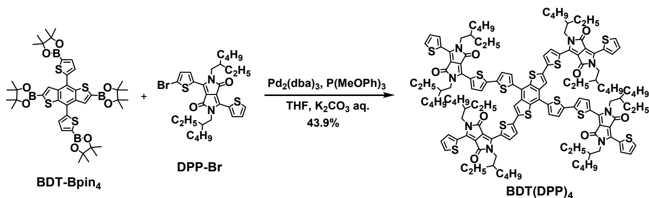
Scheme 1 Synthetic route to compound BDT(DPP) 4 .
