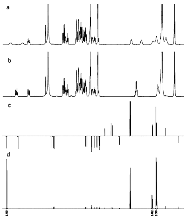
Figure 2. ^1\text{H} and ^{13}\text{C} NMR spectra of the synthesised labelled and unlabelled globotriaosylsphingosine. (a) 400 MHz ^1\text{H} NMR spectrum ( [\text{D}_4]\text{methanol} ) of labelled globotriaosylsphingosine 41b , in which the ^{13}\text{C}, ^1\text{H} coupling of the double-bond proton is apparent. (b) 400 MHz ^{13}\text{C} -decoupled ^1\text{H} NMR spectrum ( [\text{D}_4]\text{methanol} ) of labelled globotriaosylsphingosine 41b . (c) 151.1 MHz ^{13}\text{C} NMR spectrum ( [\text{D}_4]\text{methanol} ) of unlabelled globotriaosylsphingosine 41a . (d) 151.1 MHz ^{13}\text{C} NMR spectrum ( [\text{D}_4]\text{methanol} ) of labelled globotriaosylsphingosine 41b , with integration of the ^{13}\text{C} labels.
