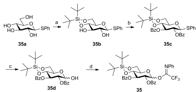
Scheme 5. Reagents and conditions: (a) t\text{Bu}_2\text{SiOTf}_2 , pyridine, DMF, –40 °C, 30 min, 77%; (b) \text{BzCl} , pyridine, room temp., 3 h, 98%; (c) NIS ( N -iodosuccinimide), TFA, \text{CH}_2\text{Cl}_2 , 0 °C, 3 h, 98%; (d) \text{ClC}(\text{NPh})\text{CF}_3 , \text{CsCO}_3 , acetone, 0 °C, 2 h, 80%.
