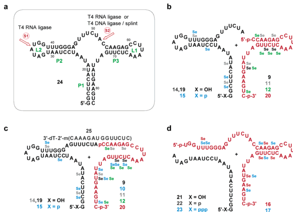
Figure 3. Enzymatic ligation of Se -modified RNA. (a) add adenine riboswitch target sequence 24 and potential sites S1 and S2 for ligation with T4 RNA ligase and T4 DNA ligase, respectively. Nucleotide numbering refers to ref 26. (b–d) Conception of the different ligation experiments: (b) T4 RNA ligations of 31 nt donor (5'-phosphate) and 40 nt acceptor (3'-OH) strands (for 3–10 Se -labels); (c) T4 DNA ligations of 31 nt donor and 40 nt acceptor strands with a 15 nt 2'-O-methyl RNA splint (for 3–10 Se -labels); (d) T4 RNA ligations of 48 nt donor and 23 nt acceptor strands (for 6–7 Se -labels).
