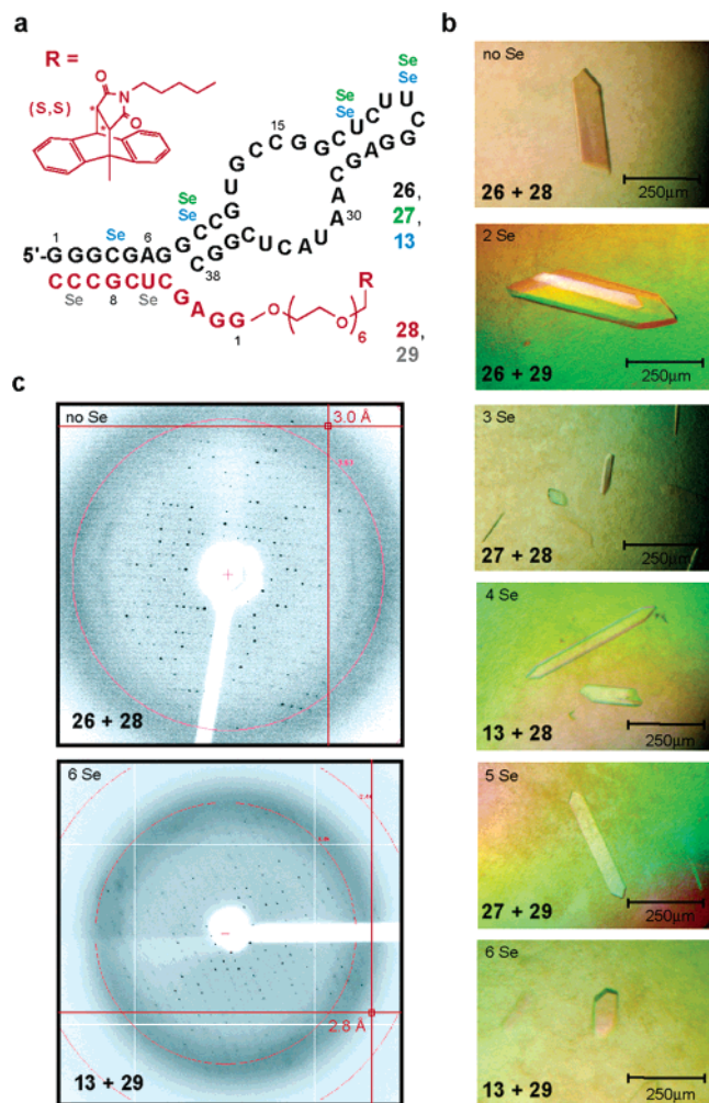
Figure 5. Crystallization of the Se -derivatized Diels–Alder ribozyme. (a) Sequences and secondary structure of the ribozyme. (b) Photographs of the typical crystals. Note that despite the different number of Se -modifications all crystals have a similar shape. (c) Diffraction patterns of the ribozyme crystals prepared either nonmodified or modified with six Se -atoms RNAs. Rotation images (oscillation 0.5°) were collected using in-house Rigaku X-ray generator (top) and beamline X25 at Brookhaven National Synchrotron Light Source (NSLS) (bottom). Note similar quality and resolution limits for both crystals.
