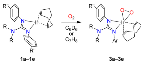
Scheme 4. Generation of (Alkene)peroxo Intermediates 3a – 3e
