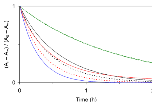
Figure 6. Time courses of the reactions of 2 mM 1a – 1f in toluene with \text{O}_2 at 0^\circ\text{C} as monitored by electronic absorption spectroscopy (path length, 0.5 cm). Color key: 1a , solid black line ( \lambda = 417 nm); 1b , dashed black line ( \lambda = 418 nm); 1c , solid red line ( \lambda = 418 nm); 1d , dashed red line ( \lambda = 419 nm); 1e , solid blue line ( \lambda = 419 nm); 1f , solid green line ( \lambda = 423 nm).
