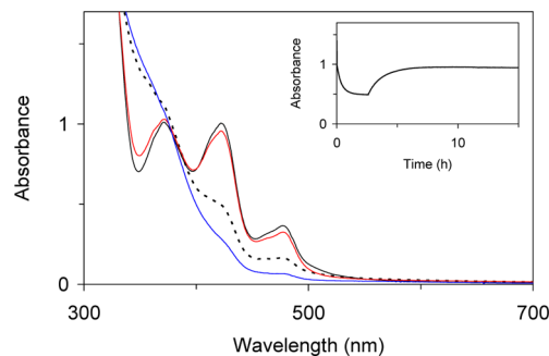
Figure 7. Electronic absorption spectra of 2 mM 1f in toluene at 20^\circ\text{C} (solid black line), the solution at maximum decay of 1f in the reaction with \text{O}_2 (dashed black line; t = 2.5 h), and 1f regenerated upon removal of \text{O}_2 (solid red line; t = 10 h; path length, 0.5 cm). The spectrum showing full decay of 1f was obtained from the reaction of 2 mM 1f in toluene with \text{O}_2 at 0^\circ\text{C} after 7.5 h (solid blue line). Inset: Time course of the reaction of 1f in toluene with \text{O}_2 at 20^\circ\text{C} and regeneration of 1f after removal of \text{O}_2 ( \lambda = 423 nm).
