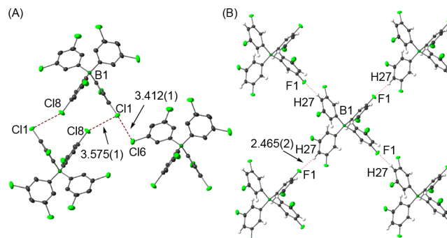
Figure 3. Interanion interactions in the solid-state structures of (A) [1\text{-NBD}][\text{BAR}^{\text{Cl}}_4] and (B) [1\text{-NBD}][\text{BAR}^{\text{F}}_4] .
