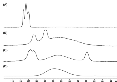
Figure 5. ^{31}\text{P}\{^1\text{H}\} SSNMR spectra (158 K) of H_2 addition (2 bar, 298 K, 1 h) to powdered crystalline [1-NBD][\text{BAR}^X_4] . (A) [1-NBD][\text{BAR}^{\text{CF}_3}_4] ; (B) [1-NBD][\text{BAR}^{\text{Cl}}_4] ; (C) [1-NBD][\text{BAR}^{\text{F}}_4] ; (D) [1-NBD][\text{BAR}^{\text{H}}_4] .
