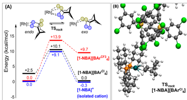
Figure 8. (A) Relative energies of endo - and exo -NBA isomers in [1-NBA] + as a function of anion and their barriers for interconversion via TS rock . (B) Detail of the structure of TS rock computed in the solid-state for [1-NBA][BAR Cl 4 ]. Method: [CP2K]PBE-D3/DZVP-MOLOPT-SR-GTH/GTH-PBE (cutoff 500 Ry).
