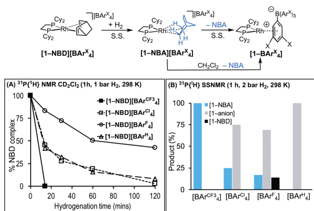
Figure 4. (A) Temporal evolution of H_2 addition (1 bar, 298 K, first 2 h) to [1-NBD][\text{BAR}^X_4] ( X = \text{Cl}, \text{F}, \text{H}, \text{CF}_3 ) as measured by the formation of [1-\text{BAR}^X_4] in \text{CD}_2\text{Cl}_2 solution. 48 (B) Selectivity of [1-NBA][\text{BAR}^X_4] formation after H_2 addition (2 bar, 298 K, 1 h) as measured by ^{31}\text{P}\{^1\text{H}\} SSNMR at 158 K.
