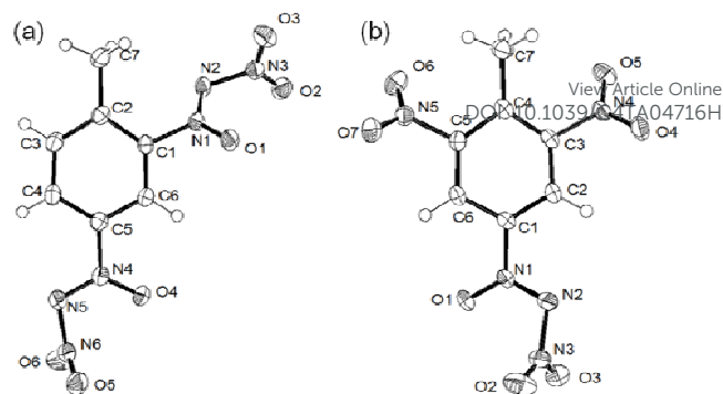
Fig. 1 Oak Ridge Thermal Ellipsoid Plot ORTEP representation of the molecular structure of 3 (a) and 4 (b). Displacement ellipsoids are shown at the 50% probability level. Selected bond length/Å: (a) C1-N1 1.47, N1-O1 1.24, N1-N2 1.28, N2-N3 1.47, N3-O2 1.21, N3-O3 1.21; (b) C5-N1 1.46, N1-O1 1.24, N1-N2 1.28, N2-N3 1.47, N3-O2 1.21, N3-O3 1.21, C1-N4 1.47, C3-N5 1.48.
