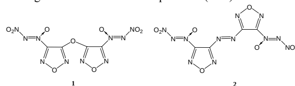
Scheme 1 Reported nitro-NNO-azoxy substituted furazan derivatives.
