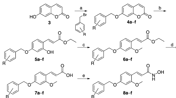
Scheme 2. Synthesis of 8a–f . Reagents and conditions: a) K 2 CO 3 , acetone, N 2 , 12 h, 75–85%; b) NaOEt, EtOH, N 2 , 6 h, 72–79%; c) DMS, K 2 CO 3 , acetone, N 2 , 12 h, 80–88%; d) LiOH, MeOH, 12 h, 92–96%; e) 1. ClCO 2 Et, Et 3 N, THF, RT, 1 h; 2. NH 2 OH·HCl, KOH, MeOH, RT, 3 h, 51–58%.
