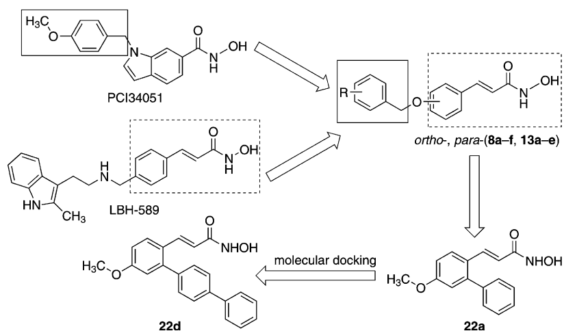
Scheme 1. Design of potent HDAC8 inhibitor 22d .
