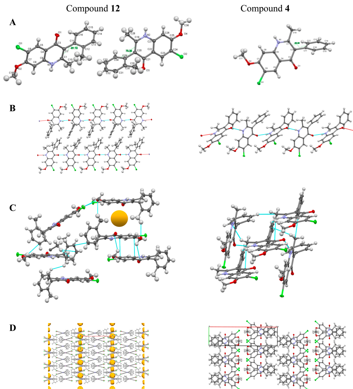
Figure 3. Crystal structures of compounds 4 and 12. (A) Asymmetric units, conformation, and numbering schemes. (B) Hydrogen-bonding schemes. (C) Packing schemes showing the disruption of \pi - \pi interactions through weak \text{CH}\cdots\text{O} and \text{CH}\cdots\pi interactions (dotted lines). The crystalline pocket in 12 is marked as a yellow sphere. Some of the molecules are omitted for clarity. (D) Packing schemes. Crystalline voids can be seen in the crystal structure of 12.
