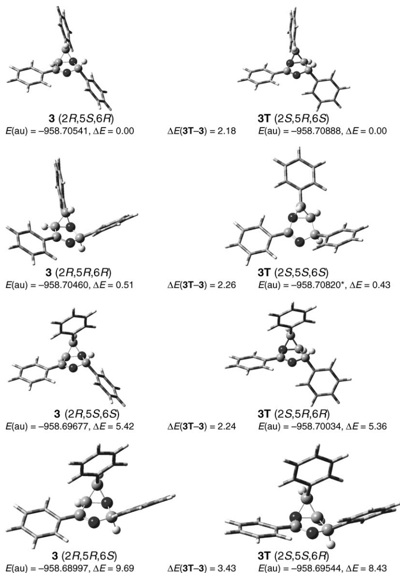
Fig. 4. Optimized geometries of the diastereoisomers of 3 and 3T , and absolute and relative stability energies computed at the B3LYP/6-31+G(d,p) level. au=arbitrary unit. ΔE in kcal/mol. Arbitrary atom numbering 1 ).
