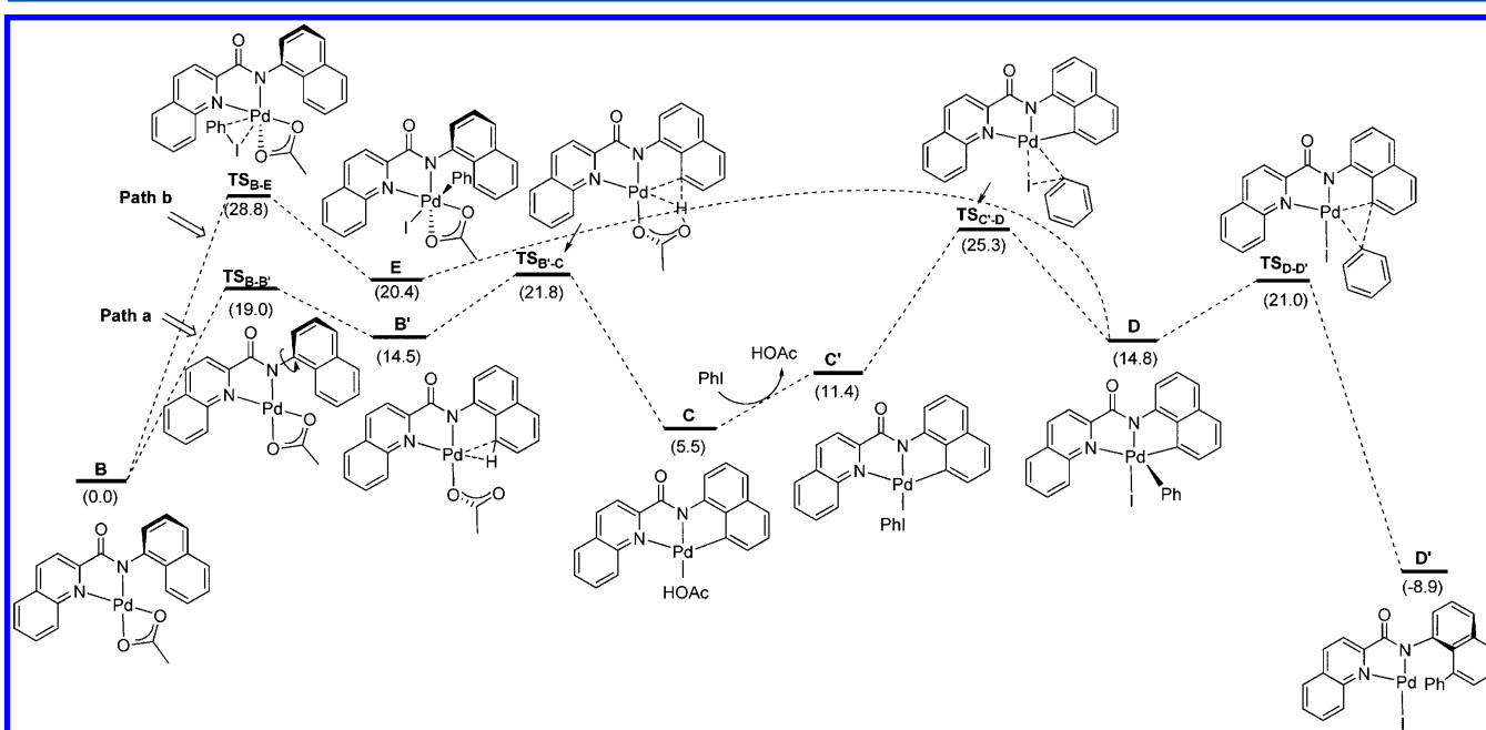
Figure 1. Potential energy surfaces of path a (sequential C–H activation/oxidative addition) and path b (sequential oxidative addition/C–H activation).
