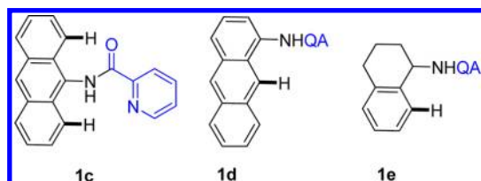
Scheme 4. Preliminary Mechanistic Studies
