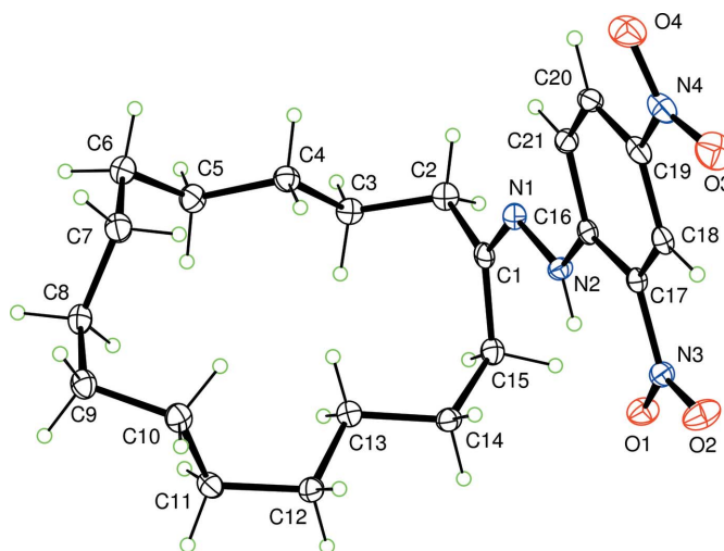
Figure 1 Displacement ellipsoid plot (50% probability) of cyclopentadecanone 2,4-dinitrophenylhydrazone, (I).
