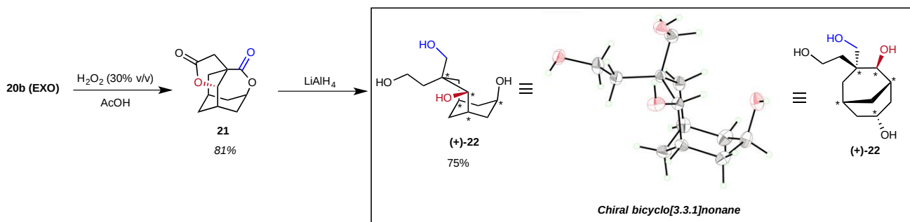
Figure 6. Synthesis of chiral tetrahydroxylated bicyclo[3.3.1]nonane core ( 22 ) via stepwise directed C–H oxidations with full enantiocontrol. Absolute configuration of (+)- 22 could not be unequivocally assigned by X-ray diffraction. Results for Mn(pdp) catalyzed oxidation of 20 are shown in Figure S5.
