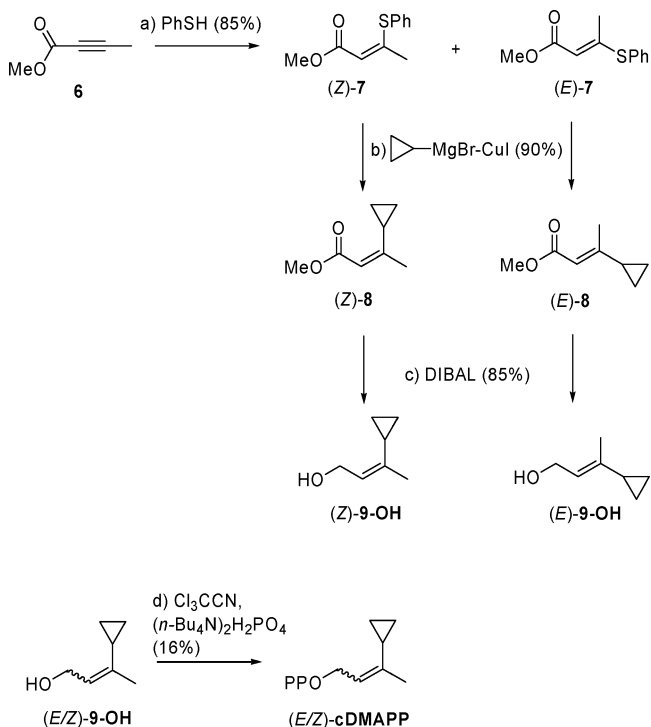
SCHEME 3. Synthesis of ( E )- 9-OH , ( Z )- 9-OH , and ( E,Z )-cDMAPP
