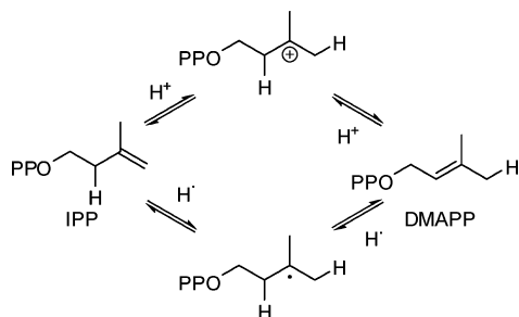
SCHEME 2. Synthesis of cIPP
