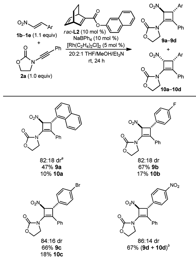
Figure 4. Rh-catalyzed [2 + 2] cycloaddition of ynamide 2a with nitroalkenes 1b–1e . Reactions were conducted using 0.30 mmol of 2 . Yields are of isolated material. Diastereomeric ratios were determined by ^1\text{H} NMR spectroscopy of the unpurified reaction mixtures. a Reaction was conducted at 40 °C for 6 h. b Ratio of 9d/10d in isolated product was 81:19.
