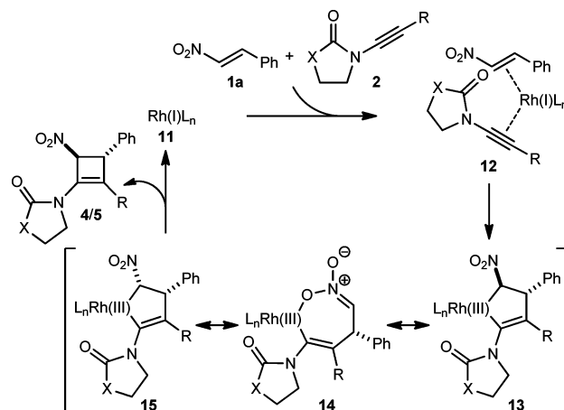
Scheme 1. Tentative Catalytic Cycle for These Reactions
