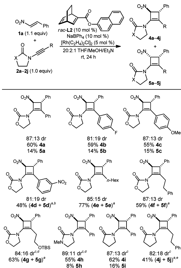
Figure 2. Rh-catalyzed [2 + 2] cycloaddition of ynamides with nitroalkene 1a . Reactions were conducted using 0.30 mmol of 2 . Yields are of isolated material. Diastereomeric ratios were determined by 1 H NMR spectroscopy of the unpurified reaction mixtures. a Inseparable mixture of diastereomers. b Ratio of 4d/5d in isolated product was 83:17. c Reaction conducted at 40 °C. d Reaction time of 6 h. e Ratio of 4j/5j in isolated product was 90:10.
