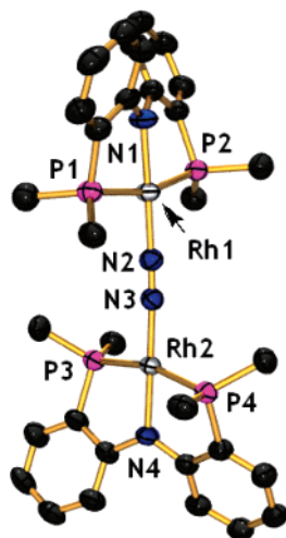
Figure 1. ORTEP drawing 29 (80% probability ellipsoids) of 19a showing selected atom labeling. Hydrogen atoms and all methyl groups are omitted for clarity. Selected bond distances (Å) and angles (deg) follow: N2–N3, 1.1191(17); Rh1–N2, 1.9035(12); Rh1–N1, 2.0358(12); Rh1–P1, 2.2818(4); Rh1–P2, 2.2808(4); Rh1–N2–N3, 178.16(12); P1–Rh1–N2, 82.18(4); P2–Rh1–N2, 81.98(4); N1–Rh1–N2, 179.52(5); P1–Rh1–P2, 163.623(14).
