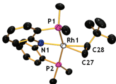
Figure 2. ORTEP drawing 29 (50% probability ellipsoids) of 21 showing selected atom labeling. Hydrogen atoms and all methyl groups are omitted for clarity. Selected bond distances (Å) and angles (deg) follow: Rh1–C27, 2.132(5); Rh1–C28, 2.189(5); Rh1–P1, 2.3220(19); Rh1–P2, 2.2964(14); Rh1–N1, 2.062(4); C27–Rh1–C28, 36.7(2); C27–Rh1–P1, 97.64(16); C28–Rh1–P1, 110.42(14); C27–Rh1–P2, 96.65(15); C28–Rh1–P2, 92.72(14); P1–Rh1–P2, 155.64(5); C27–Rh1–N1, 161.04(17); C28–Rh1–N1, 160.64(17); P1–Rh1–N1, 80.69(11); P2–Rh1–N1, 79.40(11).
