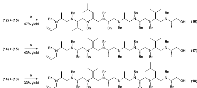
Scheme 5 Reagents and conditions: (a) (i) 1.1 eq. \text{TiF}_2\text{O} , 1.3 eq. \text{NEt}_3 , DCM, -78^\circ\text{C} \rightarrow \text{rt} ; (ii) 1.1 eq. amino alcohol, rt, 12 h.
