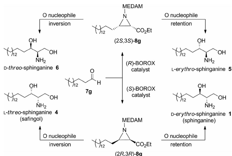
Scheme 2. Proposed syntheses of all four sphinganes.
